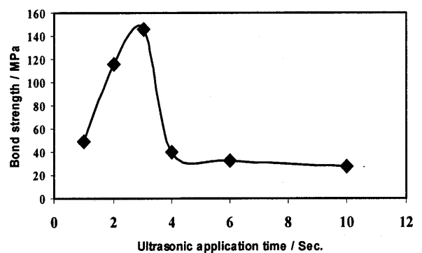
Fig. 4 Bond strength of the joints
