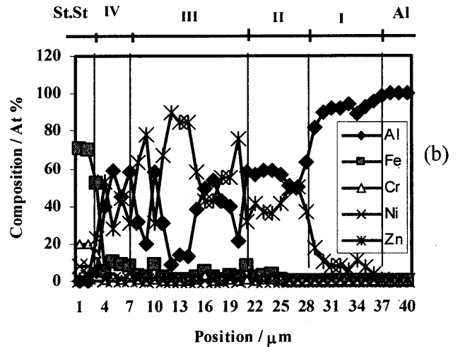
Fig. 2 SEM (a) and EPMA (b) for a joint brazed at 673 K for 2 second ultrasonic time.
