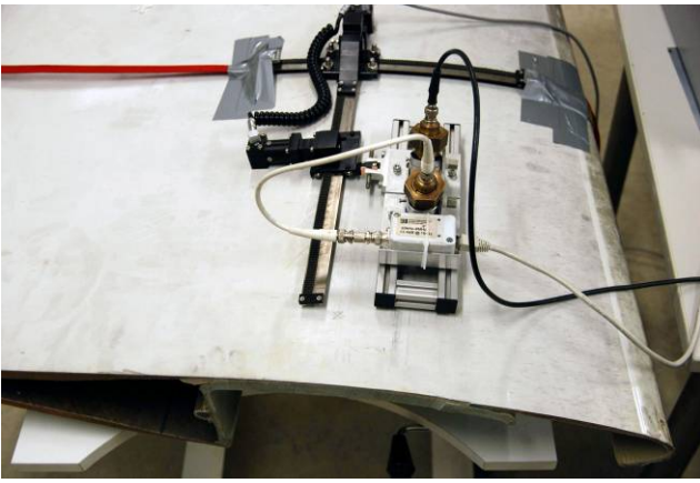
Fig.6. Photo of the air-coupled experimental set-up for wind turbine blade NDT
