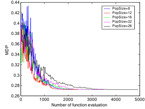
Figure 8: Searching history using different population size.
