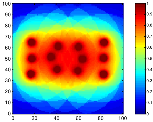
Figure 5: Sensor detectability distribution of the best sensor configuration found in one run of CMAES
