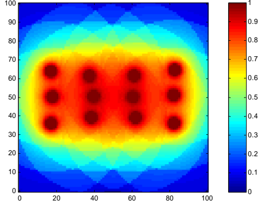
Figure 7: Another example of optimized sensor configuration
