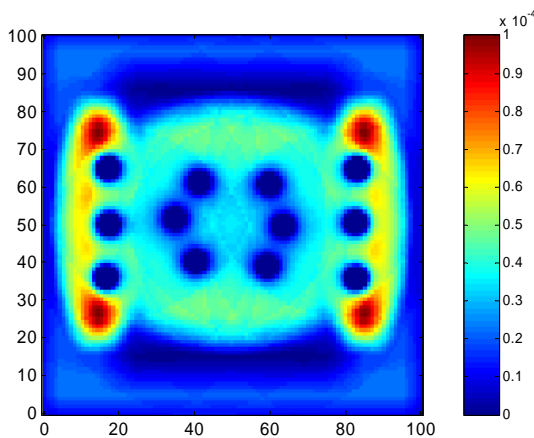
Figure 6: Damage miss-detection probability distribution
