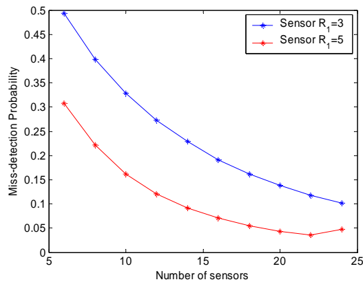
Figure 9: Relation between Miss-detection probability and the number of sensors
