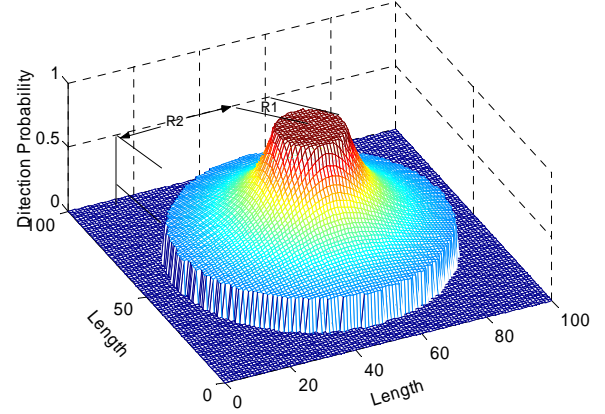
Figure 2: Sensor damage detection probability distribution
