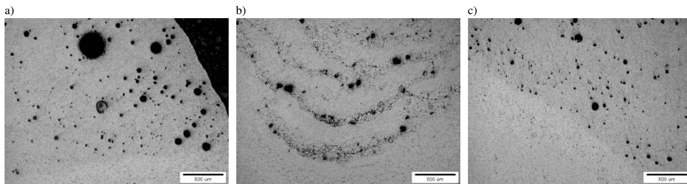
Fig. 14. Micrograph of the MIG welds: (a) without ultrasounds, (b) with the participation of ultrasounds z = 0.127 \text{ m } (1/2\lambda) , and (c) with the participation of ultrasounds z = 0.1905 \text{ m } (3/4\lambda)
