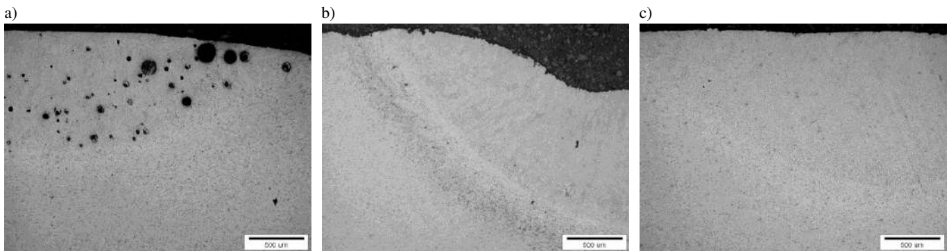
Fig. 12. Micrograph of the TIG AC welds: (a) without ultrasounds, (b) with the participation of ultrasounds z = 0.127 \text{ m} ( 1/2\lambda ), and (c) with the participation of ultrasounds z = 0.1905 \text{ m} ( 3/4\lambda )
