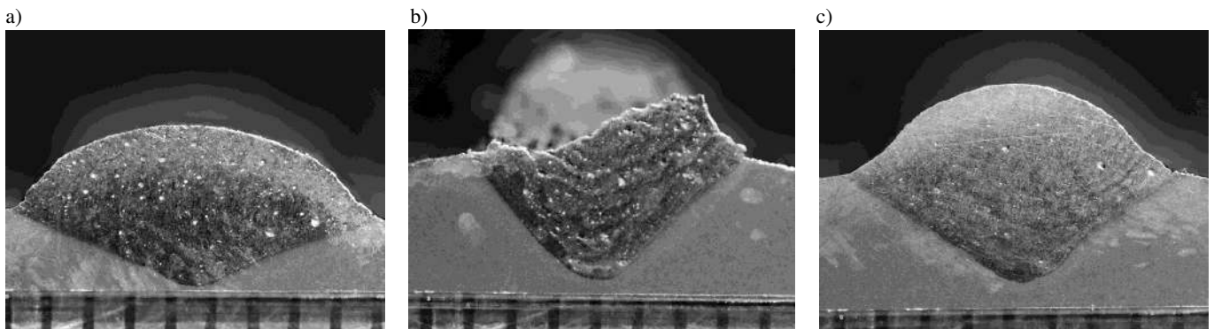
Fig. 11. Cross-section of the MIG welds: (a) without ultrasounds, (b) with the participation of ultrasounds at z = 0.127 \text{ m} ( 1/2\lambda ), and (c) with the participation of ultrasounds at z = 0.1905 \text{ m} ( 3/4\lambda ), visible scale-1 mm/div
