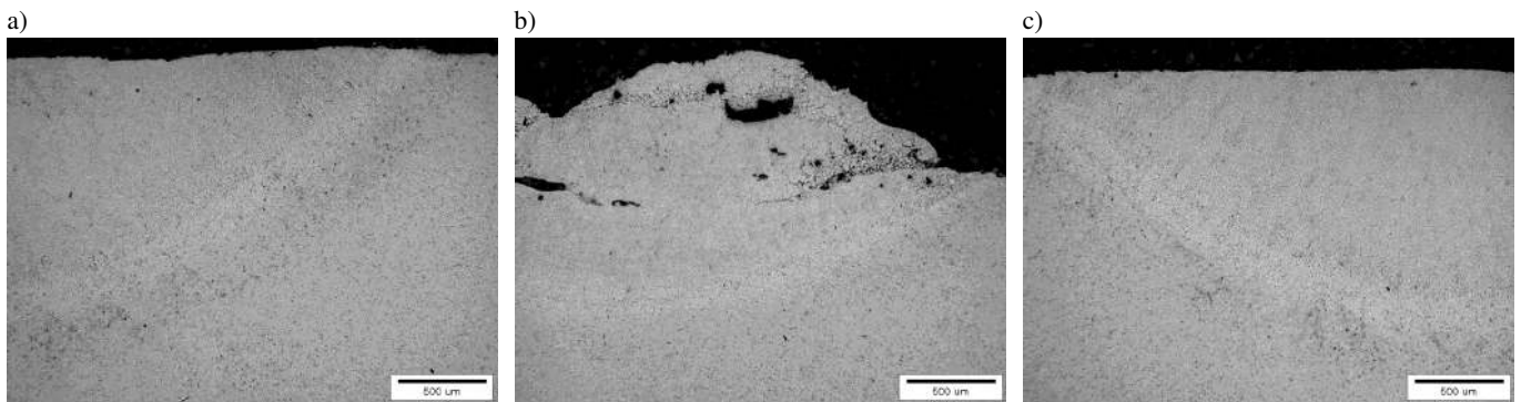
Fig. 13. Micrograph of the TIG DC welds: (a) without ultrasounds, (b) with the participation of ultrasounds z=0.127\text{m} ( 1/2\lambda ), and (c) with the participation of ultrasounds z=0.1905\text{m} ( 3/4\lambda )
