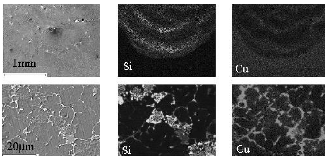
Fig. 16. Si and Cu concentrations in the MIG the cross-section weld obtained with the ultrasound assistance, z = 0.127 \text{ m}
