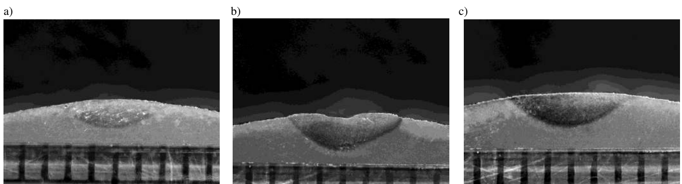
Fig. 9. Cross-section of the TIG AC welds: (a) without ultrasounds, (b) with the participation of ultrasounds at z = 0.127 m ( 1/2\lambda ), and (c) with the participation of ultrasounds at z=0.1905 m ( 3/4\lambda ), visible scale-1 mm/div
