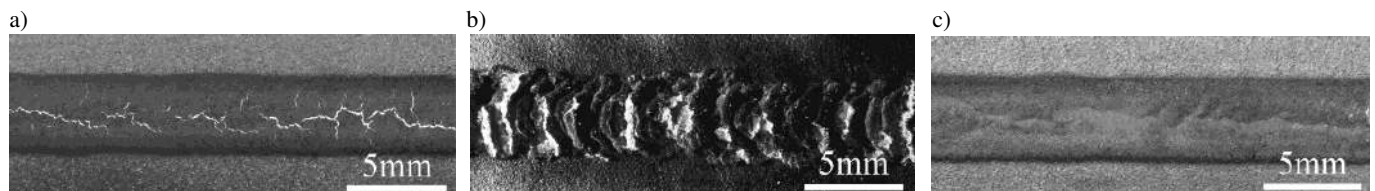
Fig. 6. TIG DC produced weld: (a) without vibrations within the (b) assisted with ultrasonic vibrations in the 0.127 m ( 1/2\lambda ) region, and (c) with vibrations in the 0.1905m region ( 3/4\lambda )
