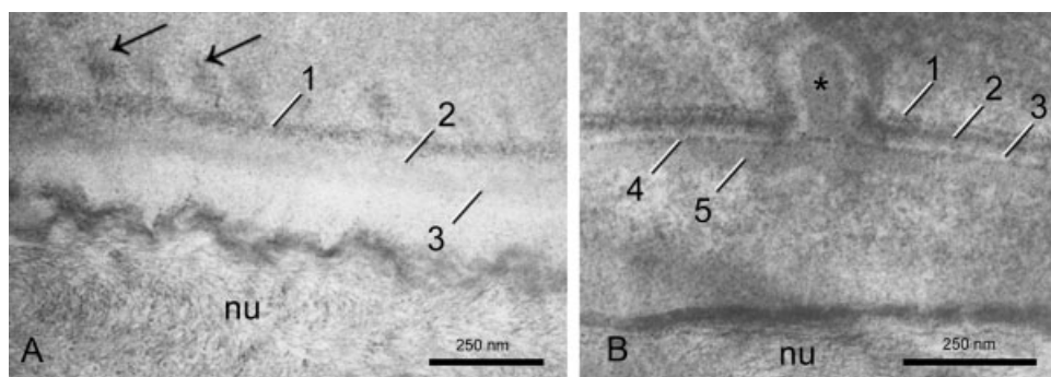
Fig. 6. The potamiscine spermatophore pellicle. TEM. (A) Larnaudia beusekomae (coenospermia). 1, outer electron-dense layer; 2, electron-lucent material; 3, inner electron-dense layer; arrows, extraspermatophoral appendages. (B) Thaiphusa sirikit (cleistospermia). 1, outer thin electron-dense layer; 2, thick electron-dense layer; 3, electron-lucent material; 4, inner thin electron-dense layer; 5, undefined electron-dense material; star, extrusion of layers 2, 3, and 5; nu, nucleus of sperm cell.
