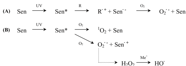
Fig. 3. Mechanisms of indirect UV-induced damage and ROS formation.
