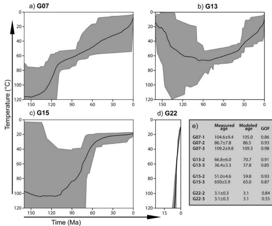
Figure 7. Thermal modeling (performed with the HeFTy software) [Ketchum, 2005] for foreland samples (a) G07, (b) G13, and (c) G15, and (d) Precordilleran sample G22. Good path envelope (supported by the data) and best fitting path are indicated with dark grey areas and a black solid line, respectively. (e) Table summarizing measured age, modeled age, and goodness of fit (GOF) for each considered grain. Age GOF provides an indication of the fit between observed and predicted data (values close to 1 are best).
