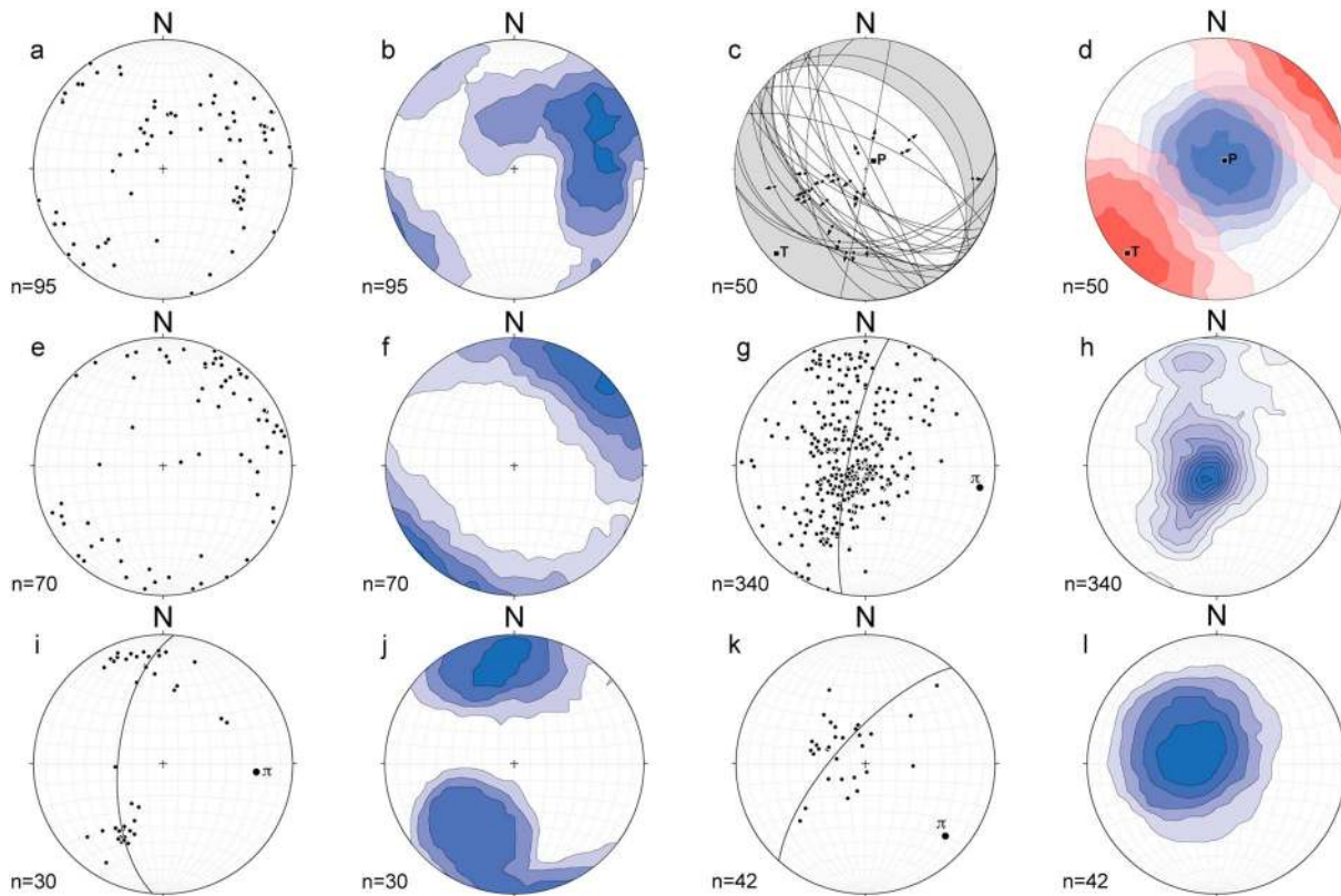
Figure 6. Orientation data (lower hemisphere, equal area projections of poles to planes drawn using Stereonet v.9.5.1 software) [Allmendinger et al., 2012; Cardozo and Allmendinger, 2013] for the Gastre area. All contours are drawn using the Kamb method with intervals at 2\sigma and significance level of 3\sigma . (a) Extensional faults showing evidence of synsedimentary/syndiagenetic activity. (b) Contour plot of data shown in Figure 6a. (c) Subset of the fault population plotted in Figure 6a, showing faults preserving slickenlines (arrows) and reliable shear sense indicators. Fault plane solution obtained by kinematic analysis performed with FaultKin v.7.4.3 software [Marrett and Allmendinger, 1990; Allmendinger et al., 2012] is also shown (grey shaded “beach ball”). (d) Contours of P (blue) and T (red) axes obtained from the kinematic analysis shown in Figure 6c. (e) Hydrothermal veins. (f) Contour plot of data shown in Figure 6e. (g) Bedding in the Cañadón Asfalto Fm. (h) Contour plot of data shown in Figure 6g. (i) Bedding from the Esperanza Syncline (refer to Figure 3). (j) Contour plot of data shown in Figure 6i. (k) Bedding from the Esperanza Anticline (refer to Figure 3). (l) Contour plot of data shown in Figure 6k. For diagrams in Figures 6g, 6i, and 6k, the best fit great circle approximating data distribution is shown, together with its pole ( \pi ) representing the statistical fold axis.
