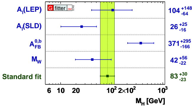
FIG. 7: Determination of the Higgs-boson mass excluding all the sensitive observables from the Gitter standard model, except for the one given [108].
