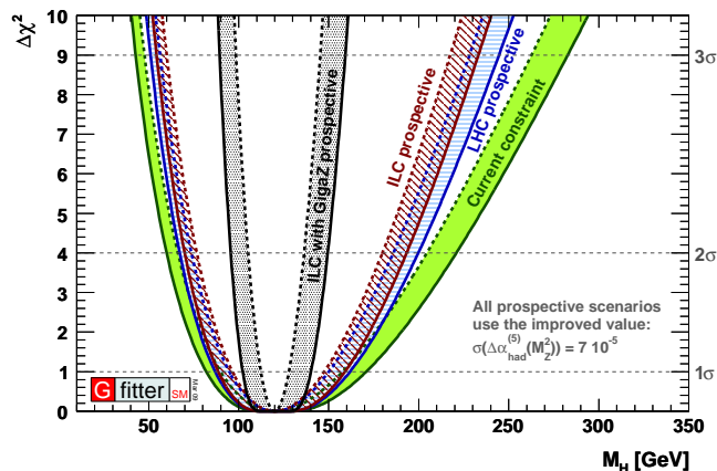
FIG. 17: Global-fit constraints on the Higgs-boson mass obtained for four future scenarios. Parabolas in \Delta\chi^2 are shown with their theoretical error bands. From wider to narrower: present constraint, LHC expectation, ILC expectations excluding and including the Giga-Z option [108].
