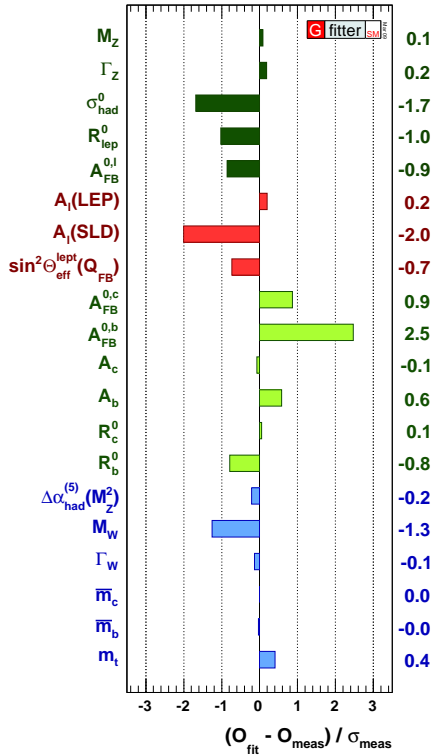
FIG. 5: Pull values comparing Gitter complete results with experimental determinations [108].
