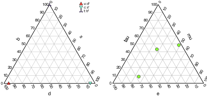
FIG. 15: Left pane: d; s; b composition of the quark flavor eigenstates d^0 (red \triangle ), s^0 (green \triangle ), b^0 (violet tripod). Right pane: e_1; e_2; e_3 flavor content of the neutrino mass eigenstates \nu_1; \nu_2; \nu_3 . The green hexagons denote central values, neglecting CP violation in the lepton sector, and with the \theta_{13} = 10^\circ [202].
