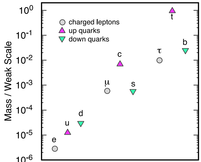
FIG. 9: Yukawa couplings y_i = m_i/(v/\sqrt{2}) inferred from the masses of the quarks and charged leptons [49].
