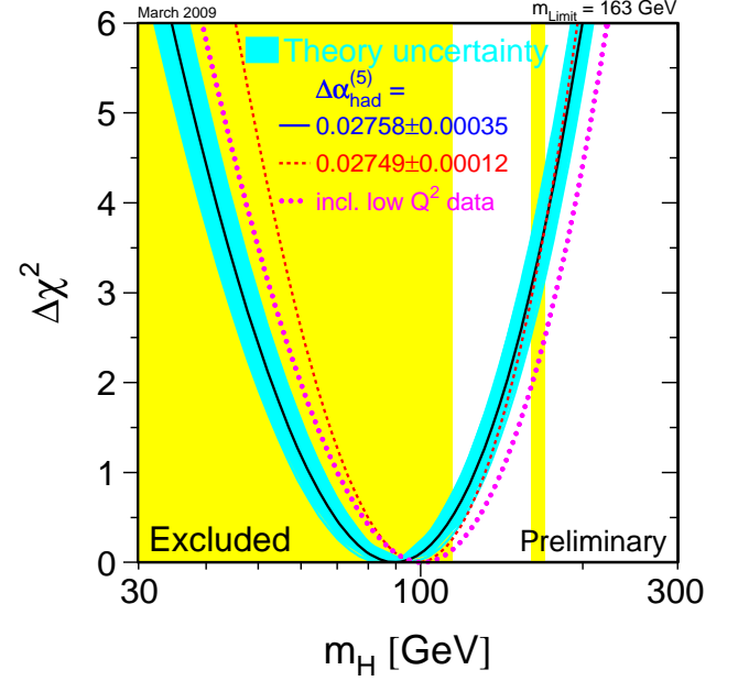
FIG. 6: \chi^2 = \chi^2_{\text{min}} + \Delta\chi^2 in from a fit to an ensemble of electroweak measurements as a function of the standard-model Higgs-boson mass. The solid line is the result of the fit. The blue band represents an estimate of the theoretical uncertainty due to missing higher-order corrections. The regions shaded in yellow denote the 95% CL lower bound on M_H > 114.4 \text{ GeV} from direct searches at LEP [117] and the Tevatron exclusion at 95% CL between 160 and 170 GeV [118]. The dashed curve shows the sensitivity to a change in the evaluation of \alpha_{\text{em}}(M_Z^2) . (From the LEP Electroweak Working Group [53].)
