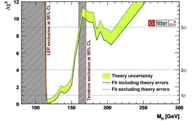
FIG. 11: \chi^2 as a function of the Higgs-boson mass for the Gitter complete fit, taking account of direct searches at LEP and the Tevatron. The solid (dashed) line gives the results when including (ignoring) theoretical errors. The minimum \chi^2 of the fit including theoretical errors is used for both curves to obtain the offset-corrected \chi^2 [108].
