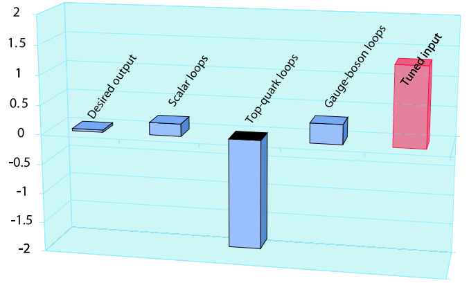
FIG. 16: Relative contributions to M_H^2 for a modest value of the cutoff parameter, \Lambda = 5 \text{ TeV} , in (5.1).
