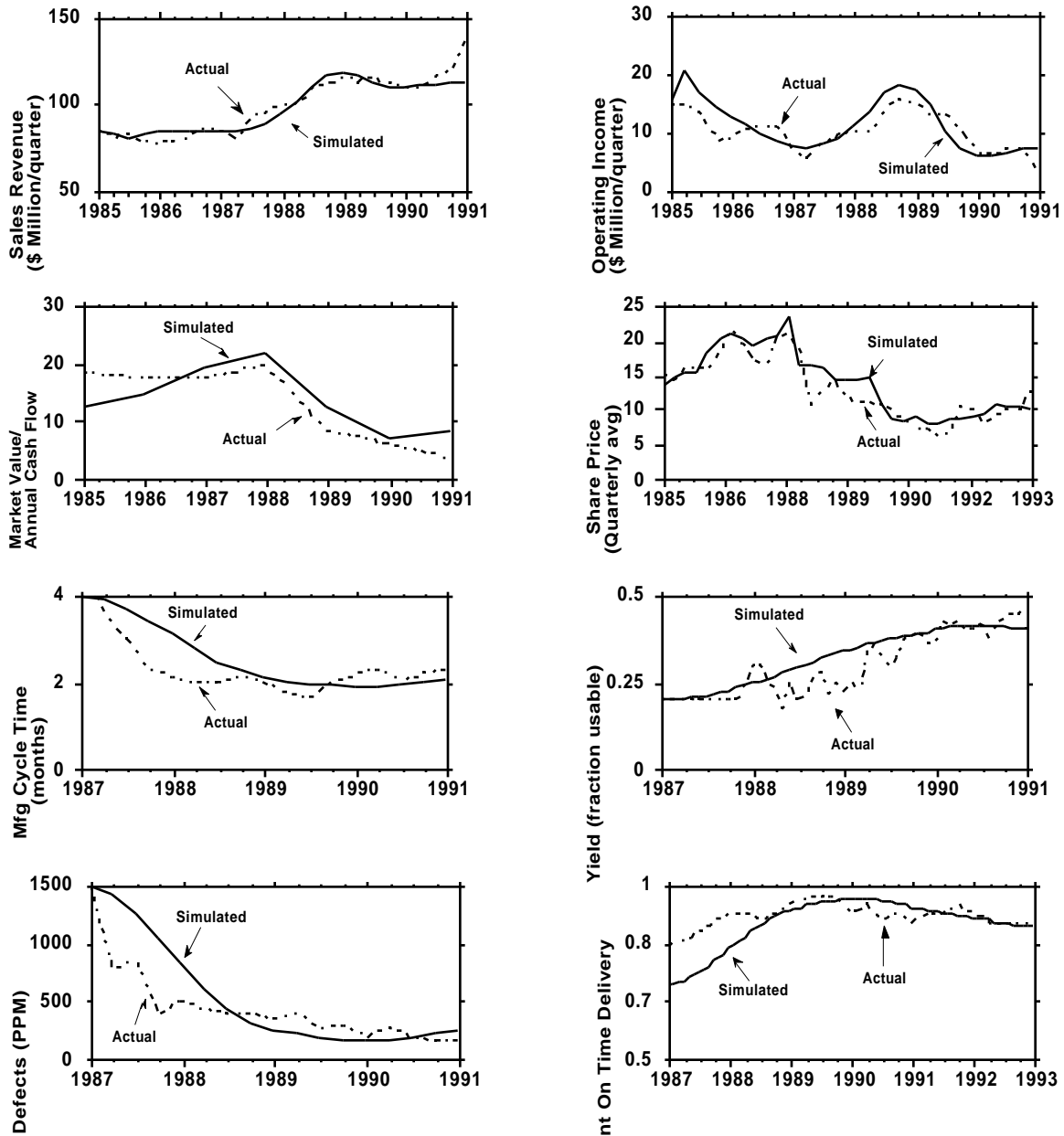
Figure 4. Selected comparisons of simulated and actual data
