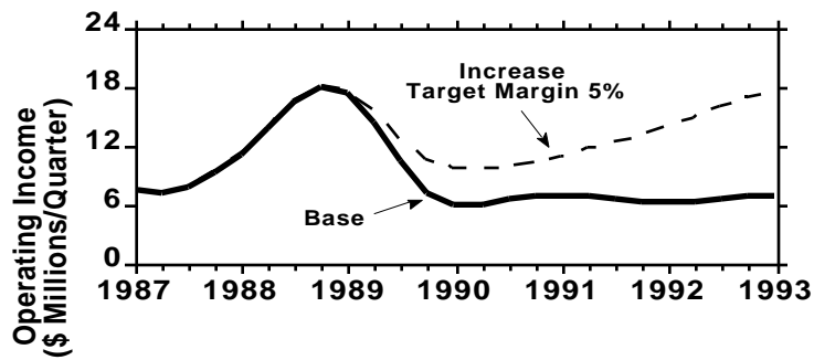
Figure 7. Raising markups to compensate for the slower reduction in indirect costs improves financial performance.
