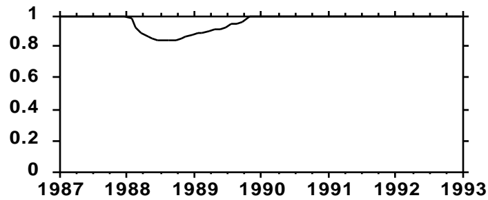
Figure 5d. Base Case: Fraction of TQM support resources allocated to manufacturing.
