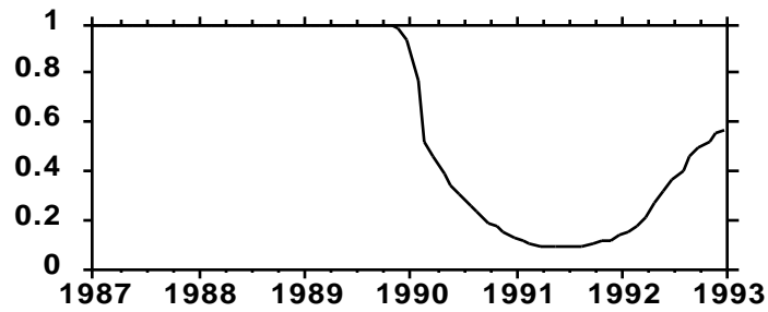
Figure 5c. Base Case: Adequacy of resources to support the TQM program.
