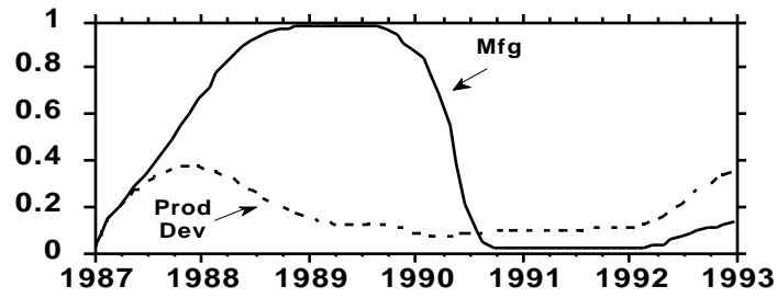
Figure 5b. Base Case: Perceived Job Security (0 = no security; 1 = no layoffs believed possible)
