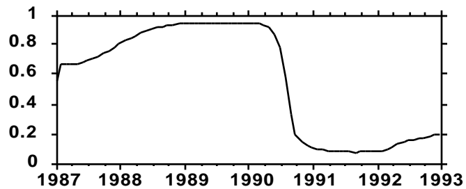
Figure 5e. Base Case: Reported and Target Product Development Time
