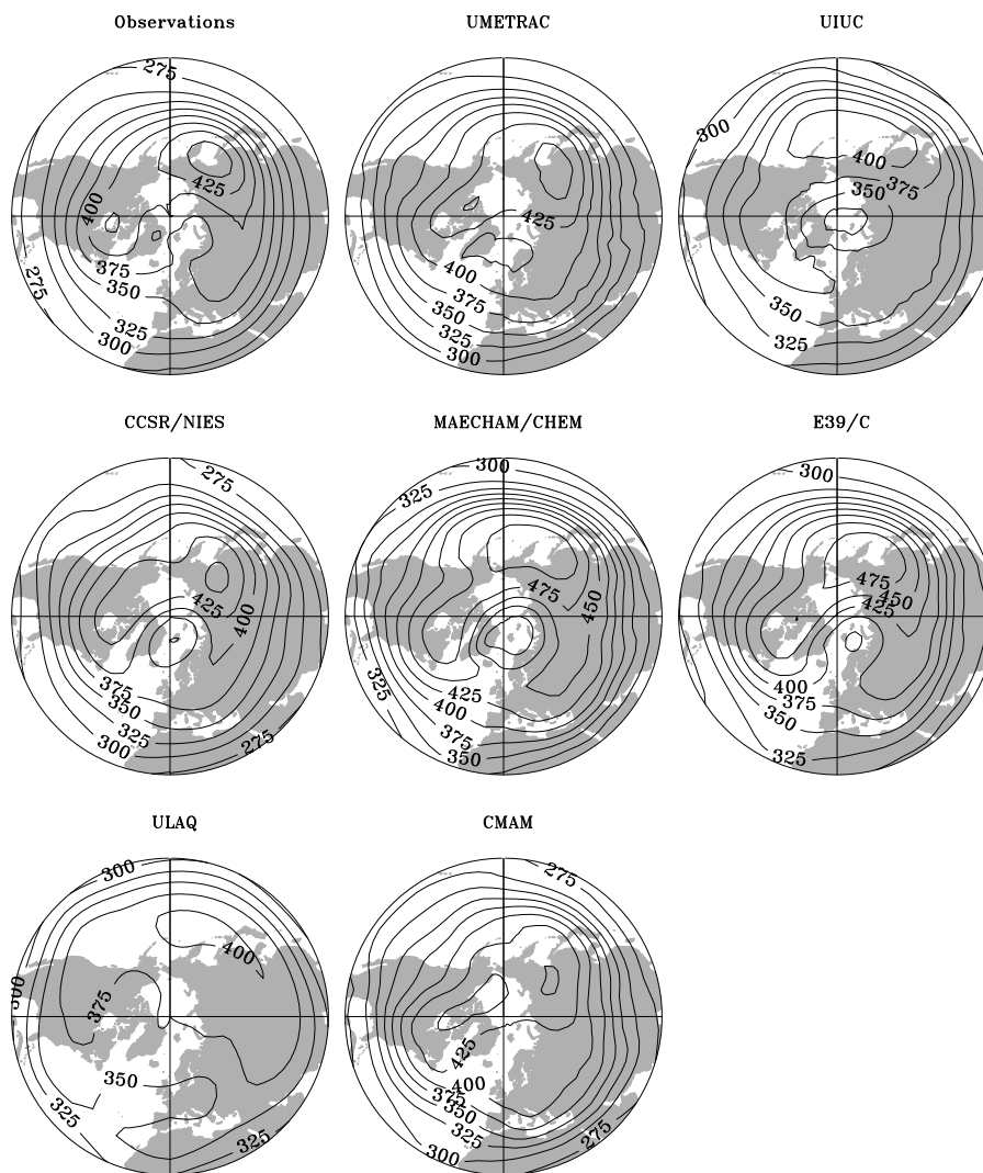
Fig. 1. Monthly mean total ozone (DU) over the northern hemisphere for the month of March for the current atmosphere for participating models. The observations are taken from a range of satellite data (see text) for the period 1993–2000. The model climatologies are as follows: UMETRAC: mean 1980–2000, CMAM: 2000 run, MAECHAM/CHEM: 2000 run, E39/C: 1990 run, CCSR/NIES: mean 1990–1999, UIUC: 1995 run, ULAQ, 1990 run.
