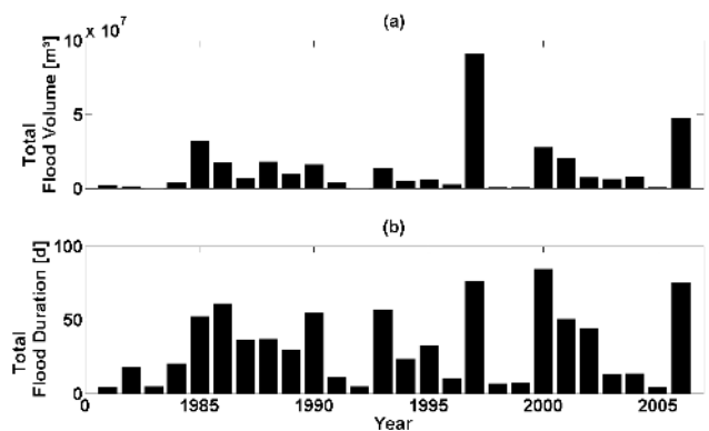
Fig. 3. (a) Flood volume and (b) duration at gauging station Schliesien from 1981 to 2006. Data are provided by the Department of Water Affairs (DWA) in Windhoek.
