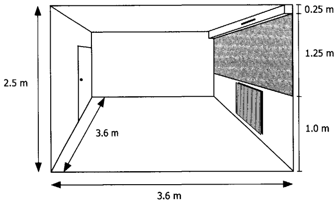
Figure 5.5 Office space 2. Internal dimensions ( l \times w \times h ) 3.6 m x 3.6 m x 2.5 m. Height of the window 1.25 m. Ventilation inlet is located above the window, 18 cm below the ceiling. The space is not furnished (empty). A hot water radiator is located below the window.
