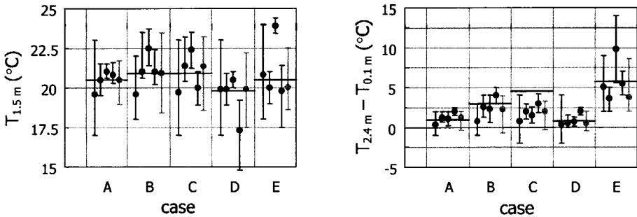
Figure 5.6 Itemwise presentation of the experts' assessment on the seed variables. The dots are their median values, the error bars show their central 90% confidence intervals. The drawn lines indicate the realizations, which were measured in a study by François et al. (1993). For each case, the results of experts 1 through 4 are shown from left to right. The rightmost, gray results show the quantile values of the item weight DM (see section 5.7.8).
