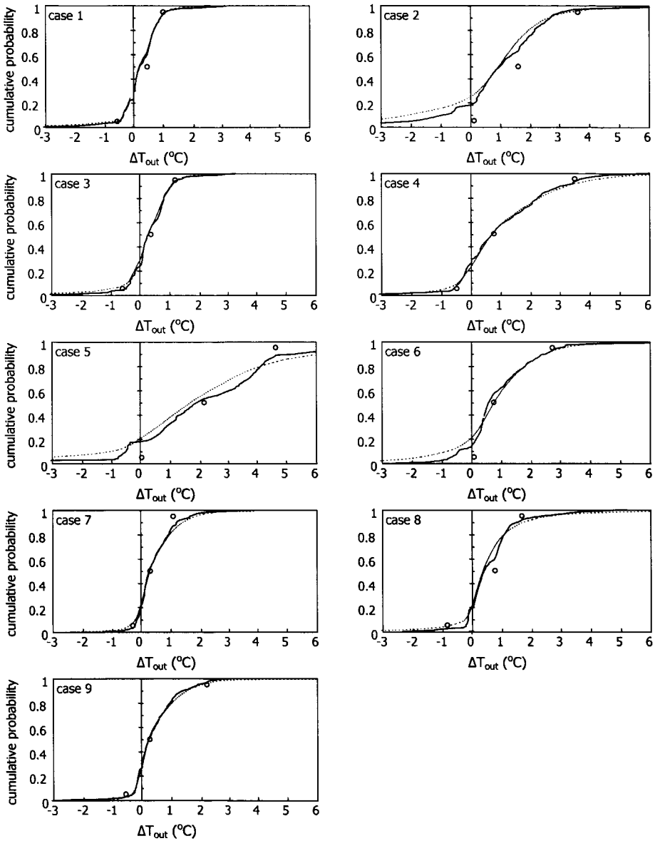
Figure 5.12 The marginal distributions for \Delta T_{outs} , resulting from the probabilistic inversion (bold, drawn lines) compared with the 5%, 50% and 95% quantile values from the item weight DM (circles). The thin, dotted lines result from the propagation of 10^5 samples, drawn from the reduced joint distribution over the target variables, i.e. the distribution represented by marginals and rank correlations only.
