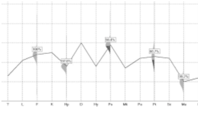
Fig. 12. Psychogram with rule conditions and fuzzified input for s = 3\% displayed.
