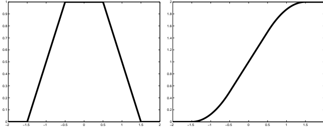
Fig. 3. Trapezoidal uncertainty and the sigmoidal quadratic-linear membership function.
