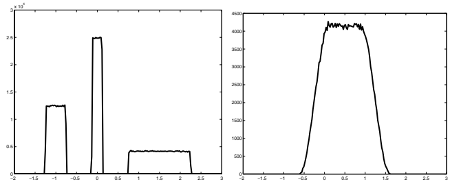
Fig. 8. 3 inputs with uniform uncertainty, but different centers and width, after convolution give semi-quadratic soft trapezoidal uncertainty distribution.
