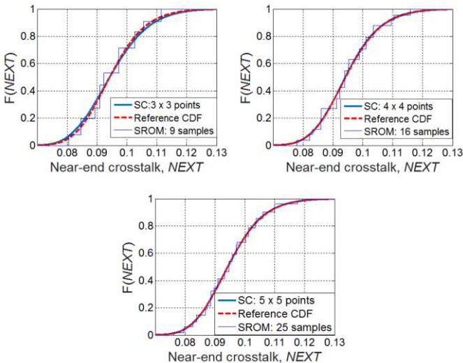
Fig. 11. The reference CDF of NEXT , the CDF approximated by the SC method (using Cubic Hermite interpolating function) with 9, 16 and 25 collocation points, and the CDF approximated by the SROMs NEXT with sizes of 9, 16 and 25.
