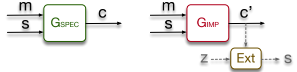
Fig. 2: Kleptography/ASA: specification G_{\text{SPEC}} takes input as the message m and the secret s , and outputs c ; whereas, the malicious implementation G_{\text{IMP}} outputs a subverted ciphertext c' which can leak the secret s exclusively to the attacker who knows z .
