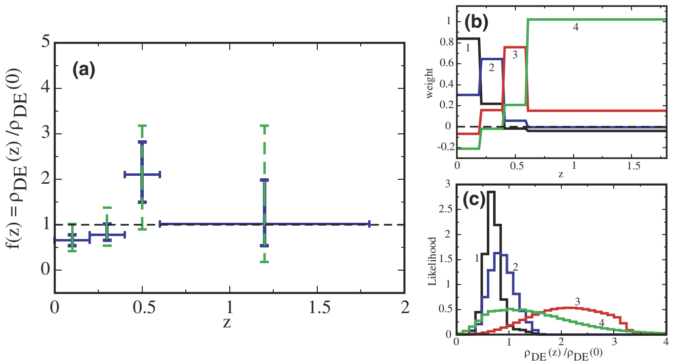
FIG. 2 (color online). Same as Fig. 1, but for f(z) \equiv \rho_{DE}(z)/\rho_{DE}(0) . Our band powers assume piecewise linear f(z) , with the exception of the band power corresponding to the largest-redshift bin, which assumes constant f(z) across that bin.
