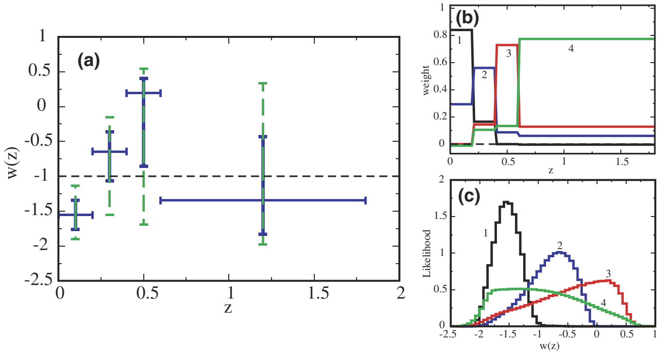
FIG. 1 (color online). Uncorrelated band power estimates of the equation of state w(z) of dark energy are shown in panel (a). Vertical error bars show the one and 2- \sigma error bars (the full likelihoods are shown in panel (c)), while the horizontal error bars represent the approximate range over which each measurement applies. The full window functions in redshift space for each of these measurements are shown in panel (b); they have small leakage outside of the original redshift divisions. The window functions and the likelihoods are labeled in order of increasing redshift of the band powers in panel (a). The window functions satisfy three of our requirements: they make the band powers uncorrelated, they are fairly well localized in redshift, and they are almost everywhere positive. In panel (a), we have used a uniform prior of 0.22 \leq \Omega_M \leq 0.38 (a Gaussian prior \Omega_M = 0.3 \pm 0.04 gives very similar results), and we have assumed a flat universe throughout.
