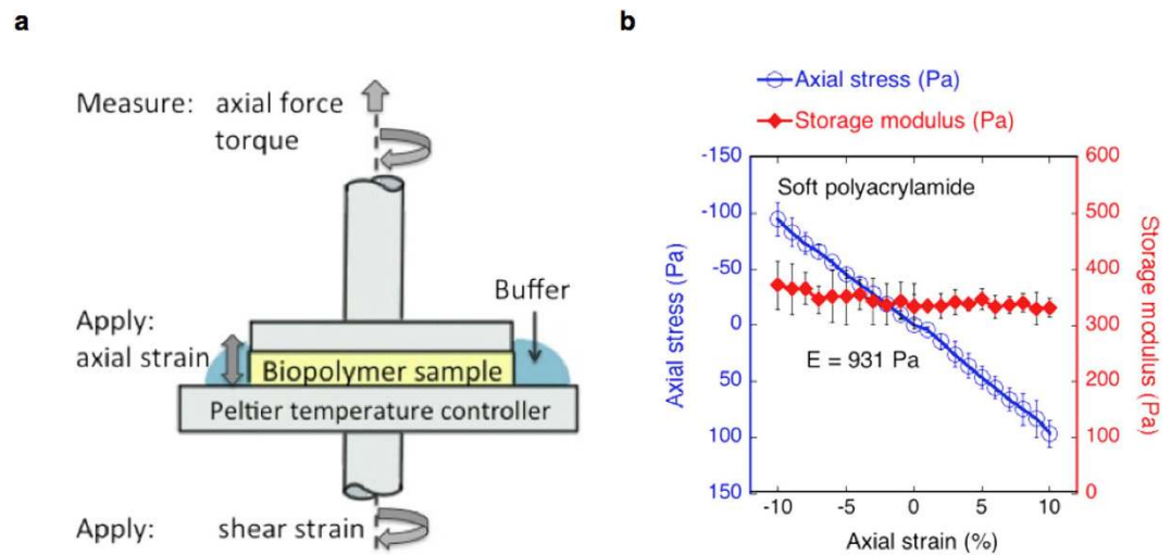
Figure 1. Experimental set-up and control experiments for multi-axial rheology method. (a) A shear rheometer is used with a parallel plate geometry. Biopolymer samples are polymerized between the plates; after polymerization buffer is added around the sample in order to prevent drying and allow free fluid flow into and out of the sample. The gap between the plates is changed to apply axial strain; the lower plate is rotated to apply shear strain. The torque and axial force are recorded. (b) The storage moduli measured with a shear rheometer and axial stress measured with a tensile tester of polyacrylamide gels (PAA). The PAA gel results show that for pure elastic linear materials the storage modulus is independent of the gap height and that the axial stress-strain curve is linear and symmetrical in compression and extension. The Young's modulus is calculated from the slope of the stress-strain curve as E = 2.8 \times G' .
