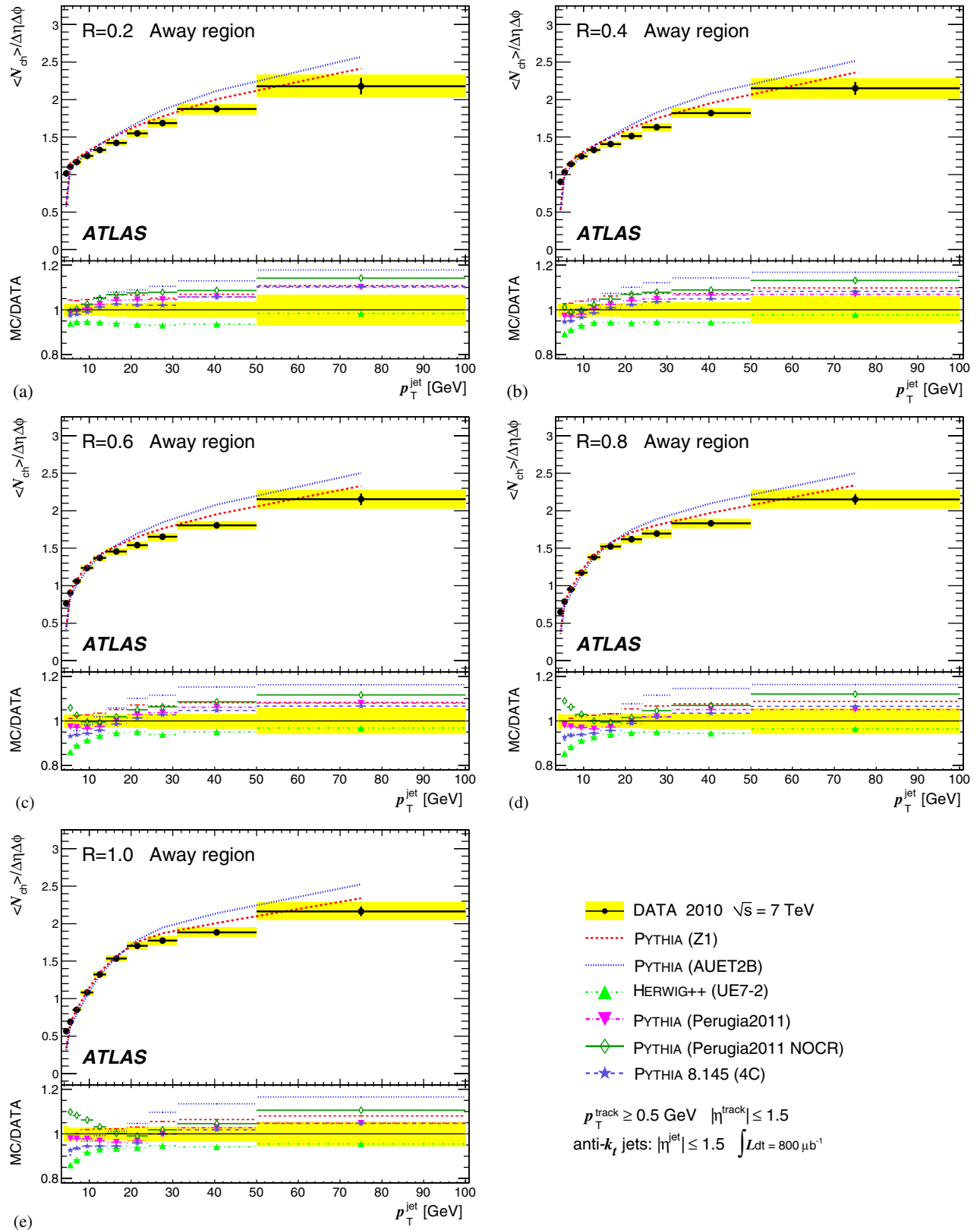
FIG. 10 (color online). The mean value, per unit \eta - \phi , of N_{ch} in the away region, as a function of p_T^{jet} (a) for R = 0.2 , (b) for R = 0.4 , (c) for R = 0.6 , (d) for R = 0.8 , and (e) for R = 1.0 . The shaded band shows the combined statistical and systematic uncertainty on the data. The data are compared to the predictions obtained with Pythia 6 using the AUET2B and Z1 tunes. The bottom insert shows the ratio of MC predictions to data for several recent MC tunes.
