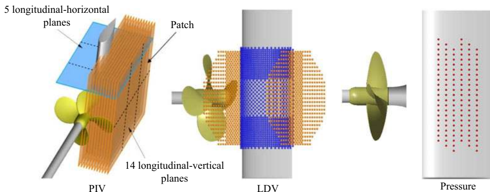
FIGURE 6. Measurement grids.
