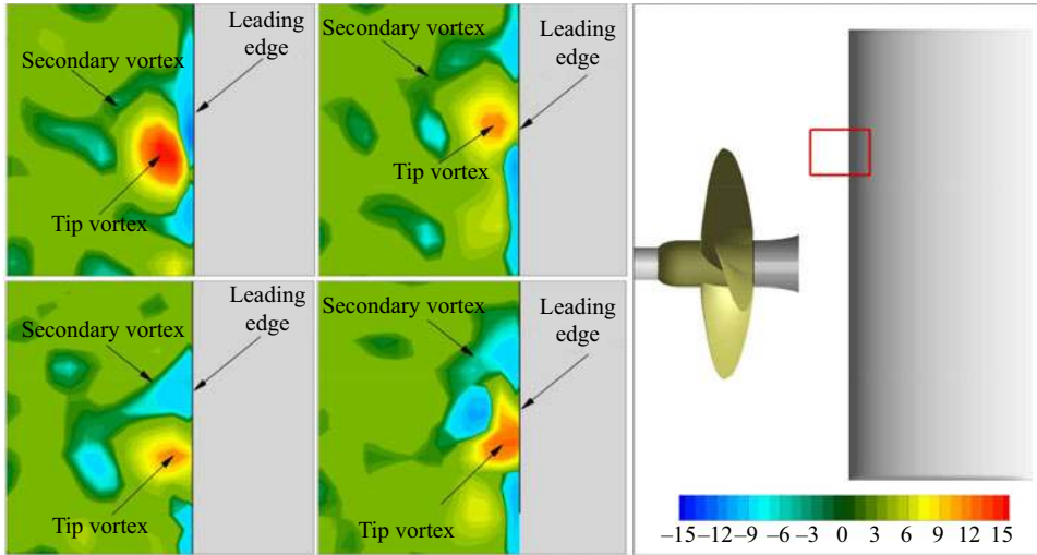
FIGURE 12. Instantaneous distributions of the out-of-plane vorticity \omega_y T during the encounter phase. Values refer to the propeller operating at J = 0.88 .
