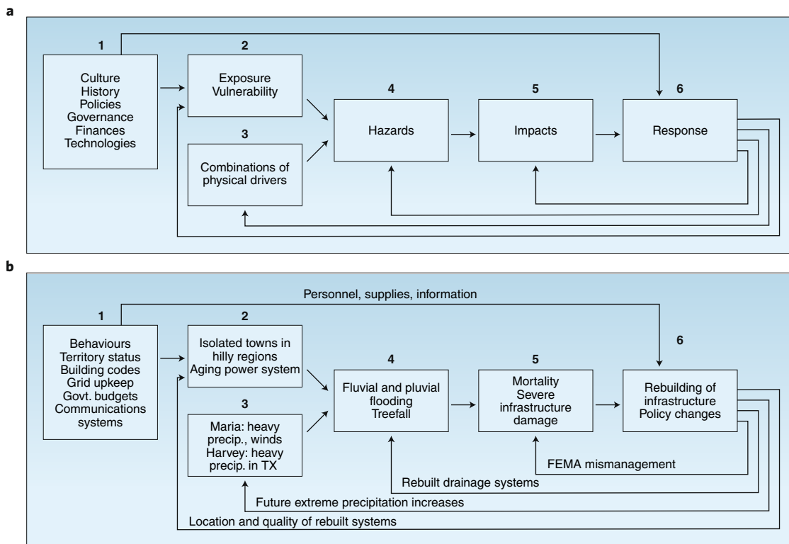
Fig. 1 | The flow of connected extremes. a , Generalized diagram of the interactions among physical and societal drivers that constitute connected extreme events. Boxes 2 and 3 together represent ‘risk’, as defined in the text. b , An illustration of a for the case of Hurricane Maria impacting Puerto Rico in 2017 following a sequence of severe tropical cyclones in the Caribbean and Gulf of Mexico. For simplicity, only one or two examples in each category are presented. Box 1 highlights behaviours 10 , territory status 20 , building codes 4 , grid upkeep 4 , government budgets 3 and communications systems 4 . Box 2 highlights isolated mountain towns 21 and the aging power system 20 . Box 3 highlights Hurricanes Maria 1 and Harvey 11 , TX, Texas. Box 4 highlights flooding and treefall 21 . Box 5 highlights mortality 21 and infrastructure damage 4 . Box 6 highlights rebuilding of infrastructure 20 and policy changes 4 . Arrows indicate FEMA mismanagement 22 , rebuilt drainage systems 25 , future extreme-precipitation increases 11 , location and quality of rebuilt systems 4 , personnel, supplies and information 23 .
