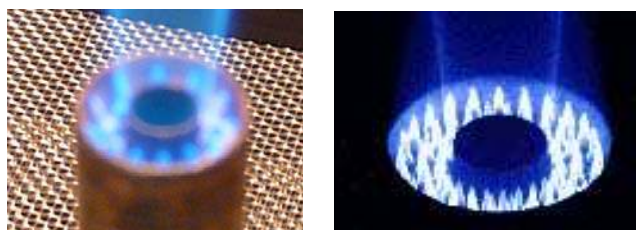
Figure 16. Photographs of the pilot flames for the “ \frac{1}{2} -scale Sydney burner,” on the left, and the actual full-scale Sydney burner, on the right.
