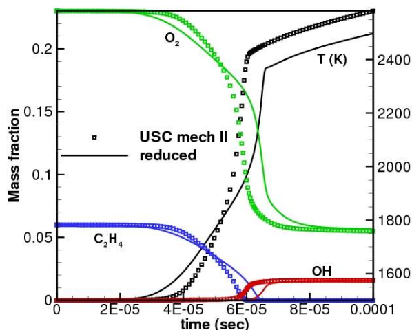
Figure 51. Comparison of CHEMKIN SENKIN results for an ethylene/air mixture when using the full USC ethylene mechanism and the new reduced ethylene mechanism.
