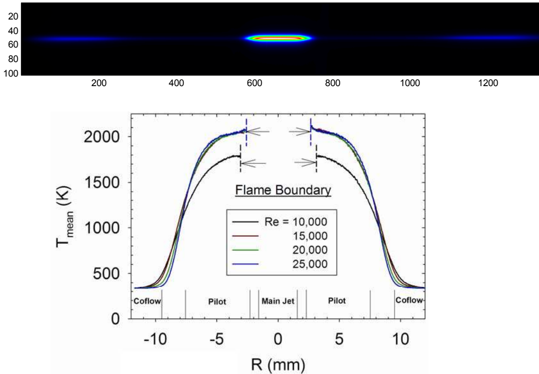
Figure 20. Sample Rayleigh scattering image (top) and derived temperature field (bottom), up to the flame boundary, 5 mm downstream from the burner lip. The anomalous profile for Re = 10,000 results from the nonlinear response of a mass flow controller for the pilot flame when used near its lower flow limit.
