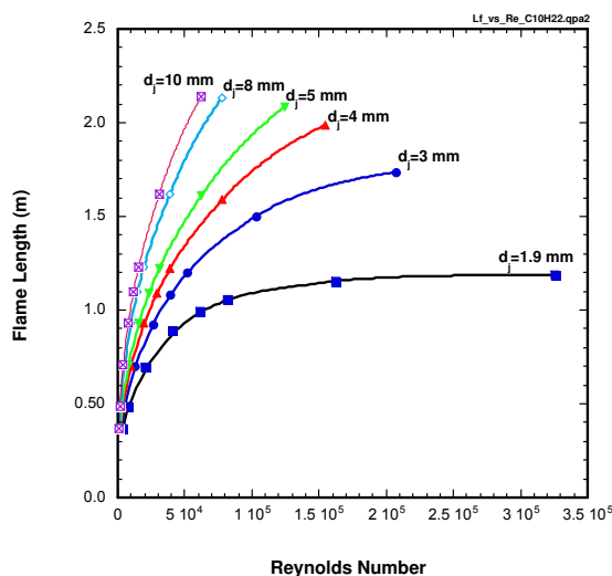
Figure 4. Calculated visible flame length of n-decane (vapor) fueled turbulent jet flame for different fuel tube diameters.
