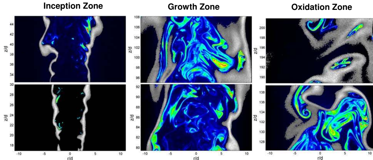
Figure 26. Evolution of OH• and soot structures within a Re = 20000 turbulent non-premixed ethylene jet flame, as revealed by simultaneous LII and OH PLIF imaging.
