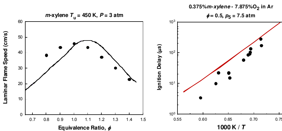
Figure 10. Comparison of experimental m-xylene-air flame speed measurements [80] (left) and ignition delay measurements [77] (right) with predictions from the detailed chemical kinetic model for SERDP JP-8 surrogate.
