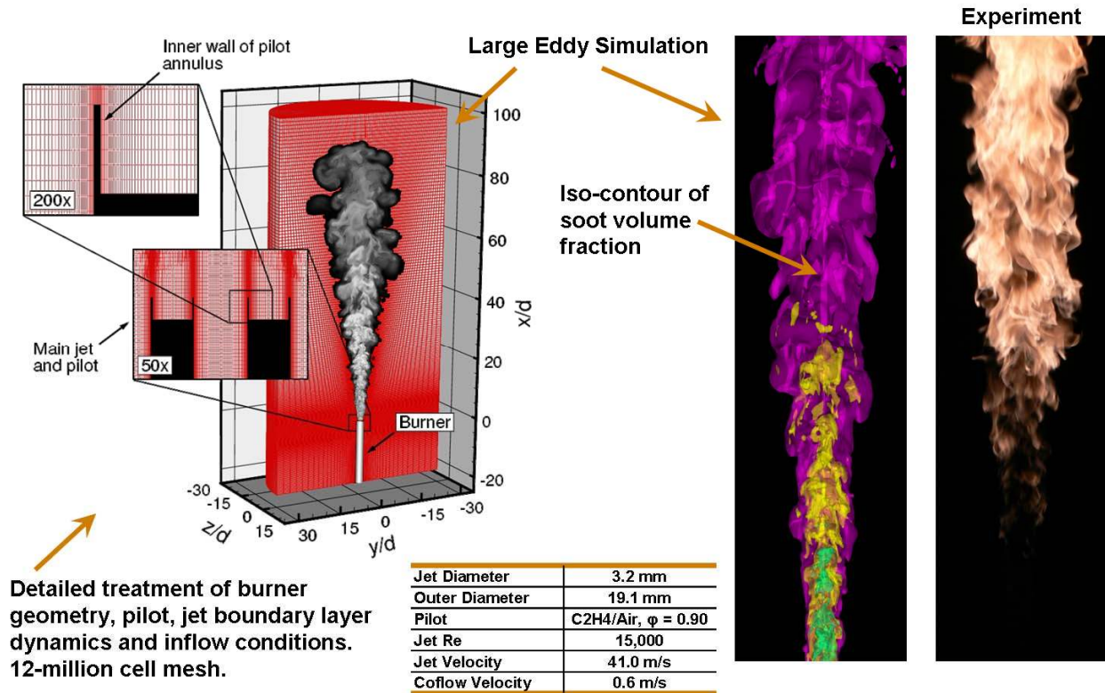
Figure 57. LES of the CRF piloted ethylene diffusion flame showing the computational domain, flow conditions and instantaneous soot volume fraction with a qualitative comparison to the experiment.
