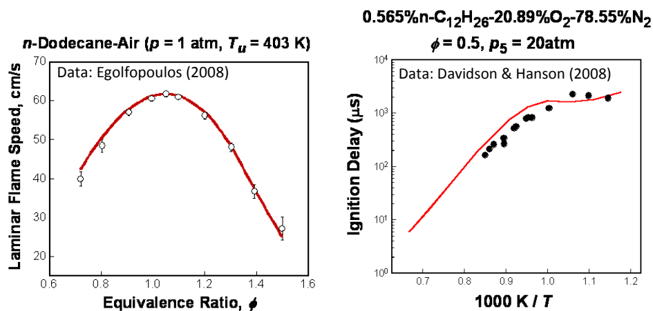
Figure 9. Comparison of experimental n-dodecane-air flame speed measurements [78] (left) and ignition delay measurements [79] (right) with predictions from the detailed chemical kinetic model for SERDP JP-8 surrogate.
