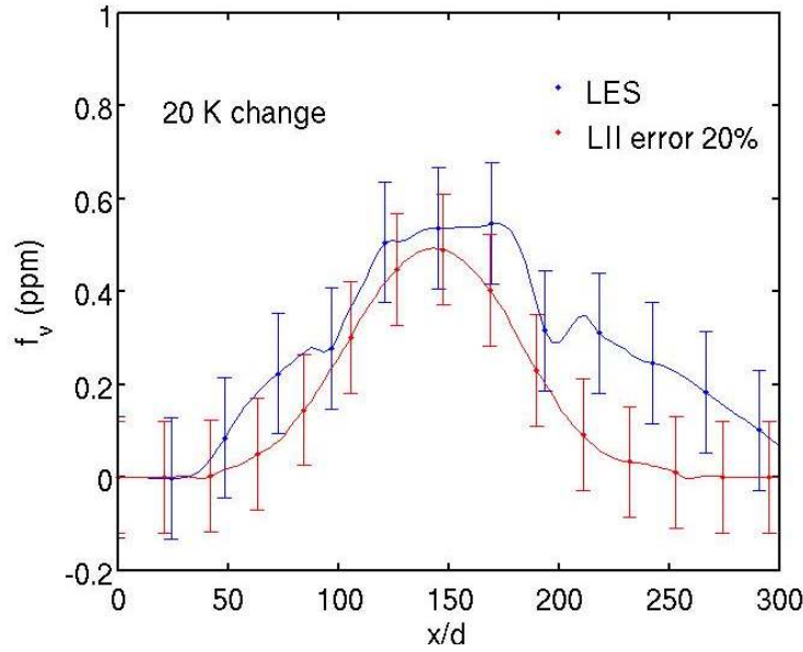
Figure 58. Soot volume fraction versus axial distance along the centerline of the burner.
