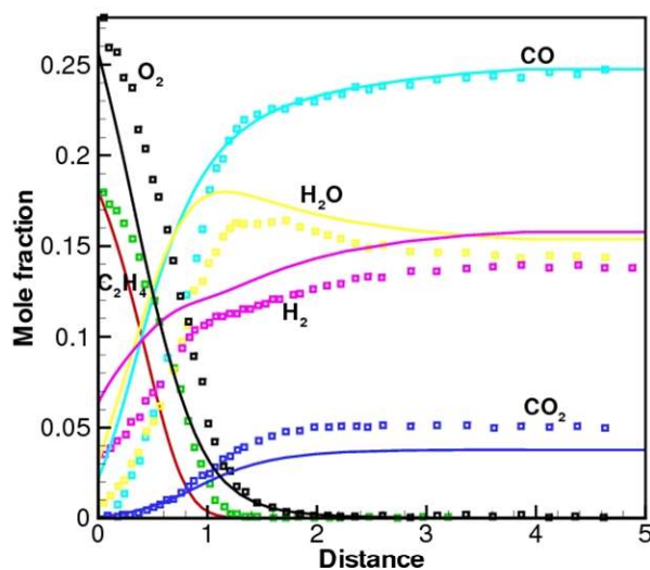
Figure 52. Comparison between CHEMKIN PREMIX calculations using the reduced ethylene chemical kinetic mechanism and experimental measurements above a flat flame burner [103]: p=20 Torr, C_2H_4/O_2/50\% Ar, \phi=1.9 ).
