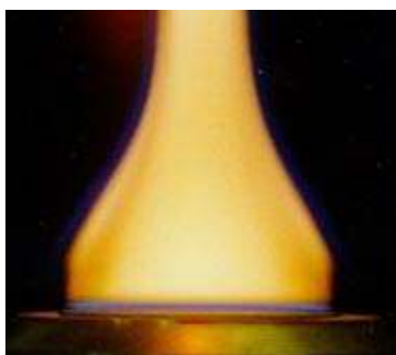
Figure 2. Photograph of typical sooting ethylene premixed flat flame, stabilized on a McKenna burner.
