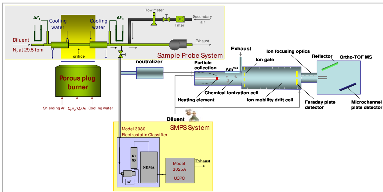
Figure 3. Schematic diagram of flat flame soot sampling and analysis by SMPS or thermal desorption chemical ionization mobility mass spectrometry (TD-CIMMS).
