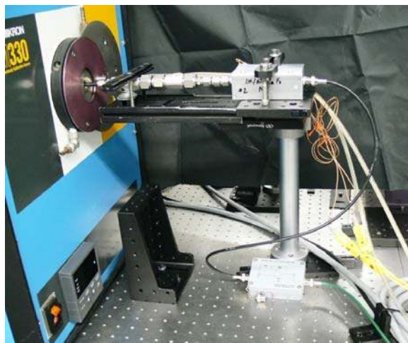
Figure 46. Photograph of radiometer, with water-cooled light pipe attached, positioned at exit of a blackbody source, to calibrate the radiometer output.
