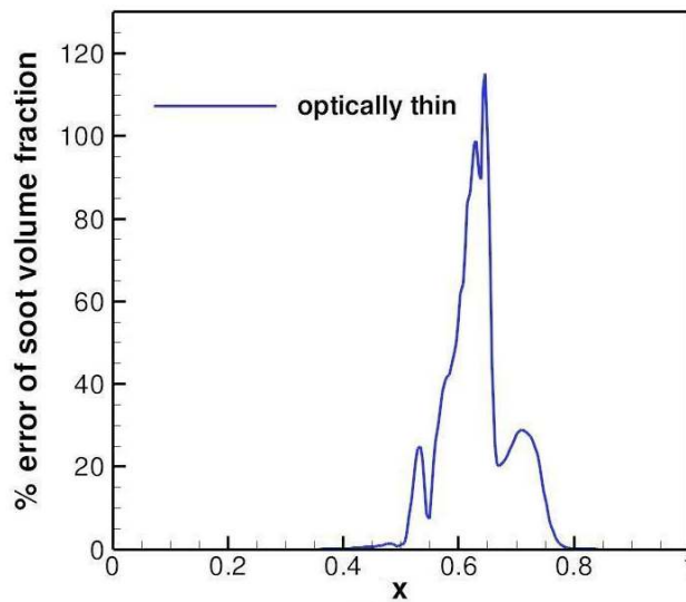
Figure 56. The calculated error of soot volume fraction between the optically thin radiation model to the P_1 gray model, where P_1 gray model is assumed to be the correct solution.
