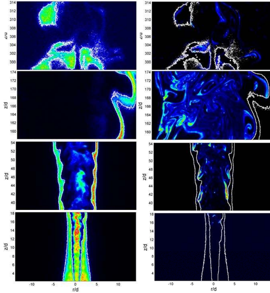
Figure 27. Evolution of OH• and soot within a Re = 20,000 turbulent non-premixed JP-8 surrogate jet flame, as revealed by simultaneous LII and OH• PLIF. Images on the left show LIF from OH• and PAH (in interior regions, particularly low in flame), whereas images on the right show soot LII, with boundaries of OH• in white.
