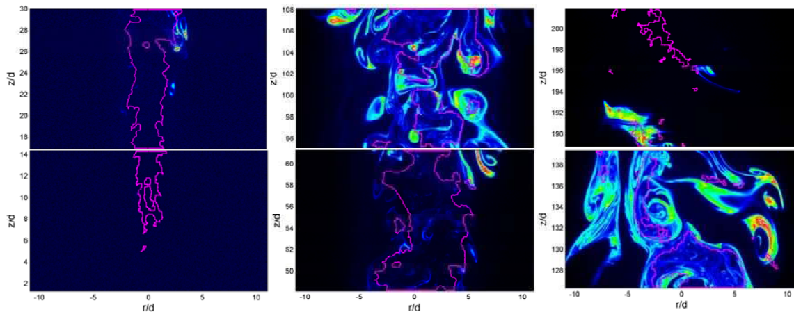
Figure 28. Evolution of PAH and soot structures within a Re = 20,000 turbulent non-premixed ethylene jet flame, as revealed by simultaneous LII and PAH PLIF imaging. The images show soot LII, with boundaries of PAH denoted in magenta.
