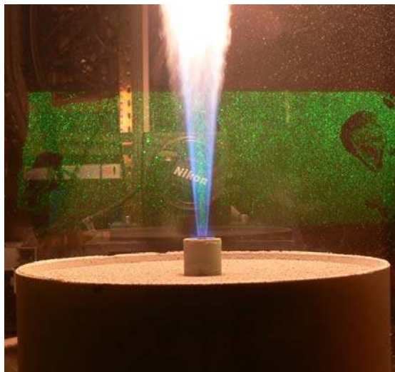
Figure 50. Photograph of the base of the ethylene jet flame when applying PIV to the seeded flow within the fuel jet and in the surrounding coflow air.
