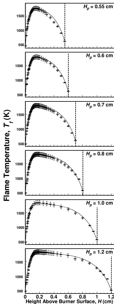
Figure 14. Comparison of measured and radiation corrected gas temperature (symbols) and calculated temperature profiles in an ethylene flame as a function of distance from the burner surface. The sampling plate position relative to the burner surface is marked by the dashed lines. The computation assumes a stagnation flow field.
