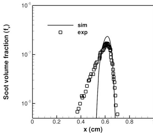
Figure 54. Comparison of diffusion flame experiment from Wang et al. [105].
