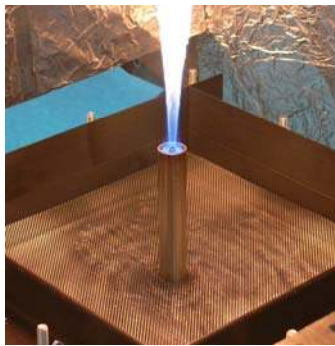
Figure 24. Photograph of the flame base of SERDP JP-8 surrogate TNF flame.
