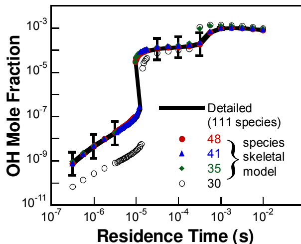
Figure 8. Test of skeletal models in adiabatic PSR. The error bars are the uncertainty of the detailed model and were determined by a spectral expansion method [76].
