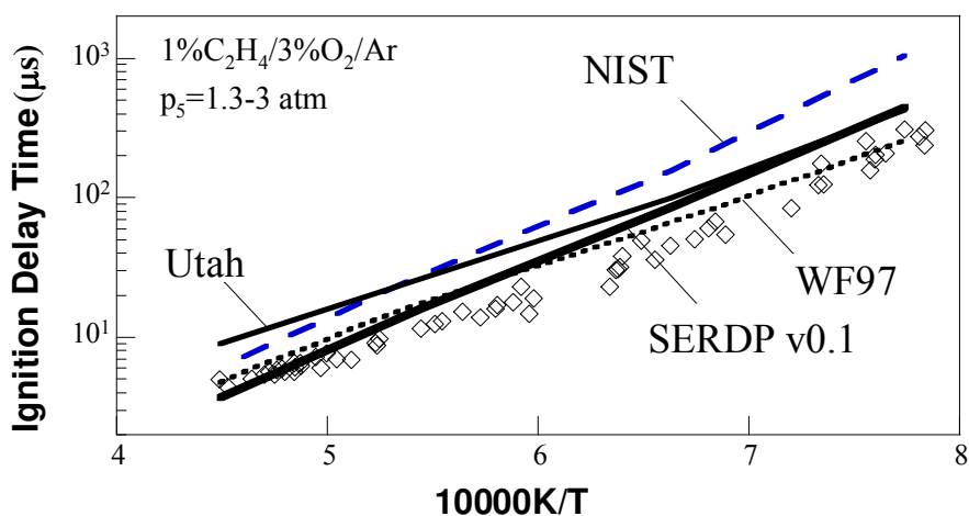
Figure 6. Experimental (symbols) and computed (lines) ignition delay times behind reflected shock waves. Experimental data are taken from ref. 75. The ignition is measured by the onset of \text{CH}^* chemiluminescent emission.
