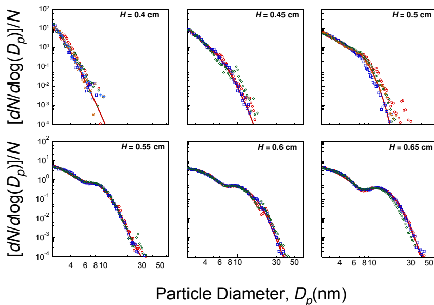
Figure 12. Evolution of PSDFs measured for ethylene flat flame with a maximum temperature of 1660 K. Symbols are experimental data and lines are fits to data using a bi-lognormal distribution function.
