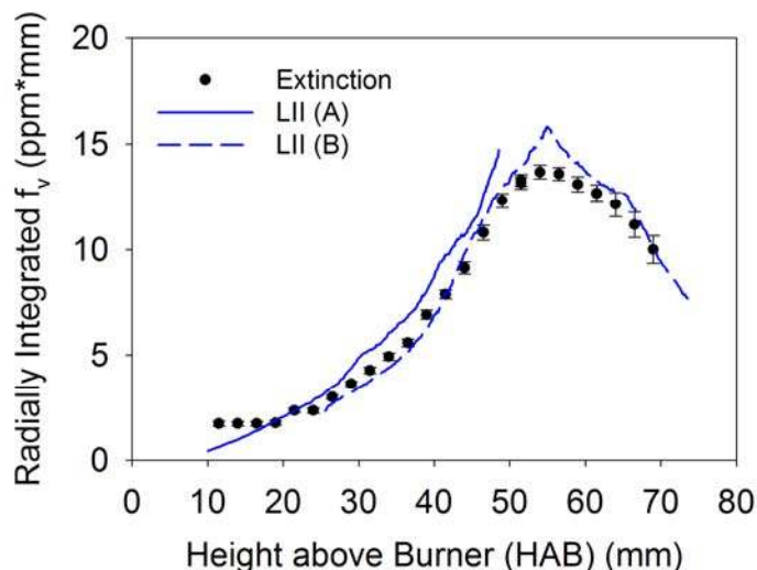
Figure 30. Axial profile of soot volume fraction integrated across the canonical ethylene jet flame measured by laser extinction and LII. A and B indicate results from LII images obtained at two different heights.
