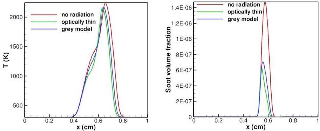
Figure 55. Unsteady, unstrained ethylene-air diffusion flame showing soot volume fraction which compares the optically thin radiation model, P_1 gray radiation model and no radiation model.
