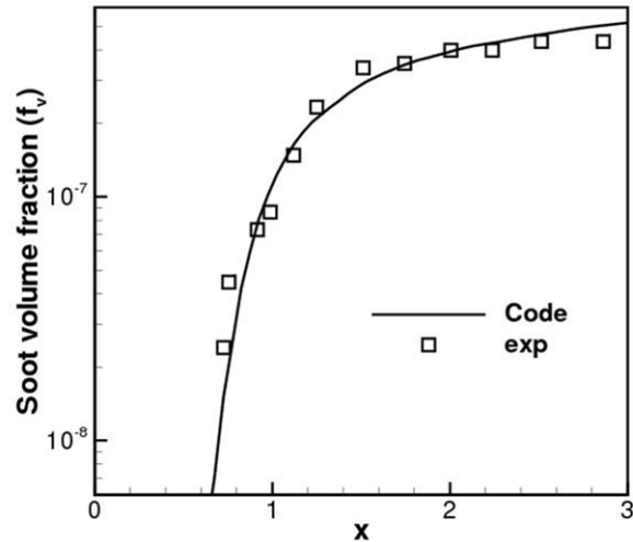
Figure 53. Comparison of premixed experiment from Appel et al. [104].
