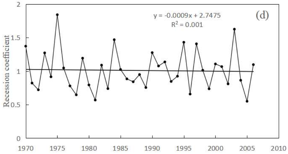
Fig. 13 Monthly recession coefficient (RC) of discharge in the study area during 1970-2006
