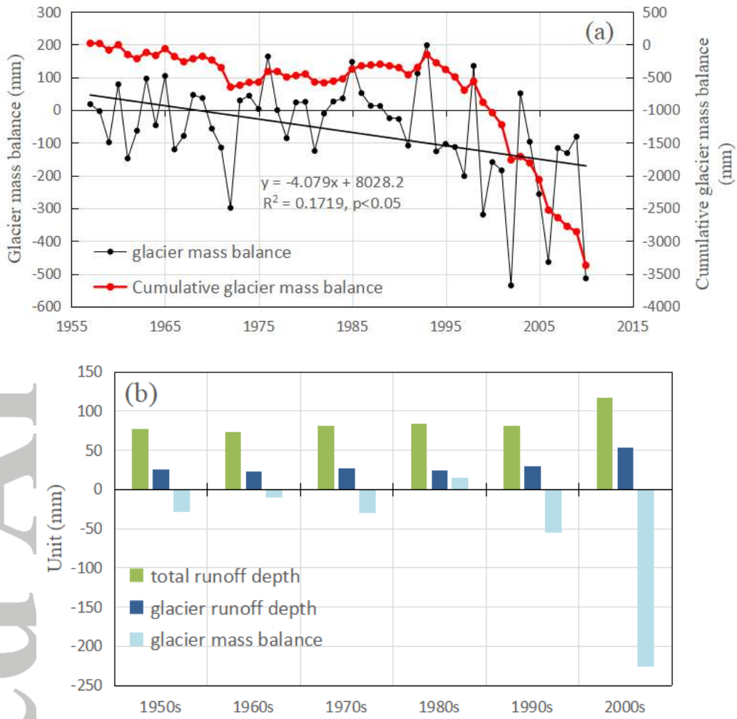
Fig. 7 (a) Variations of glacier mass balance and cumulative glacier mass balance, (b) Variations of total runoff depth, glacier runoff depth and glacier mass balance in the upstream of Shule River Basin during 1957-2010
