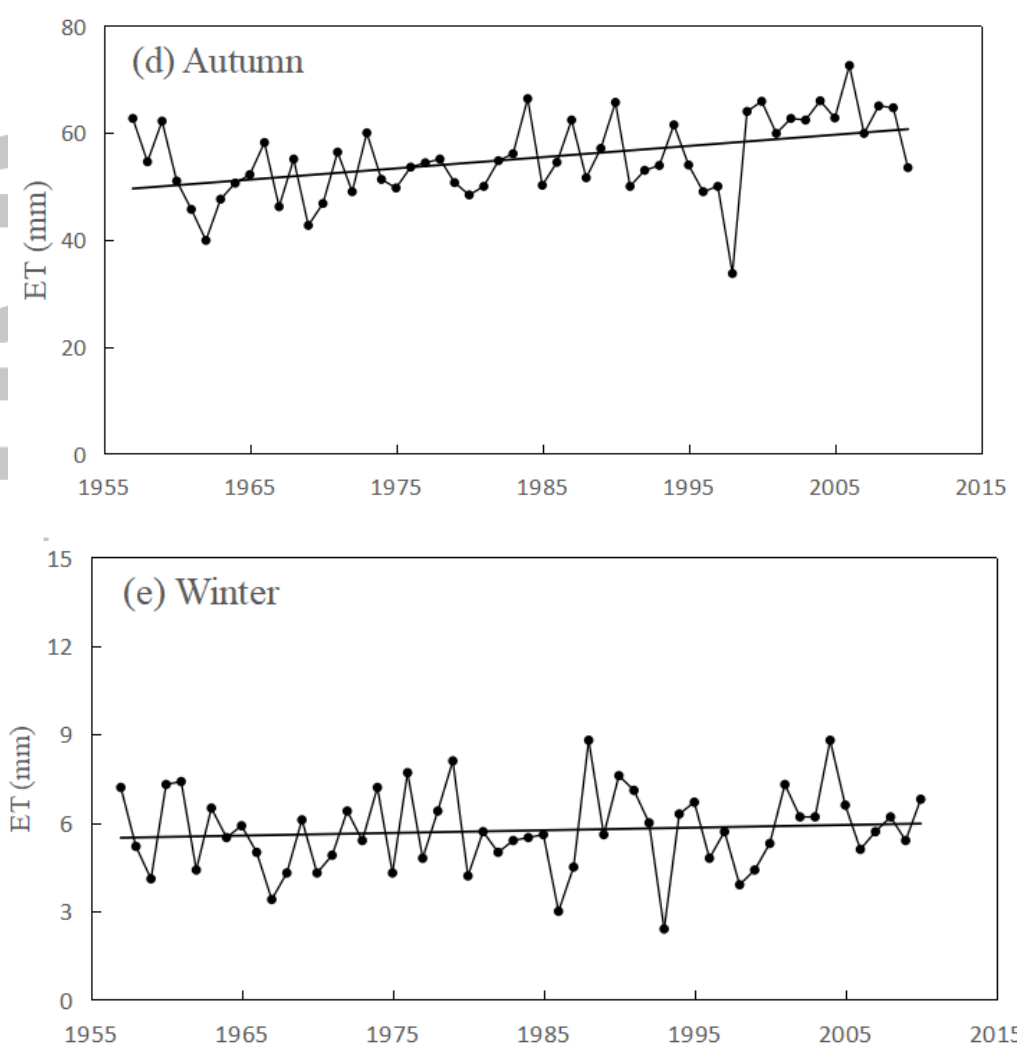
Fig. 8 Variations of (a) annual ET and (b-e) seasonal ET in the Tuole station during
