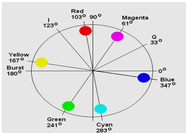
Figure 12: YIQ representation [16].
