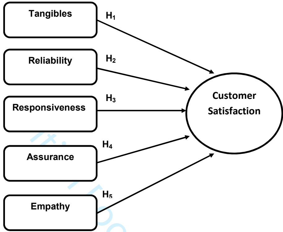
Figure 1 Conceptual Framework
