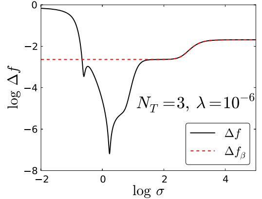
FIG. 10: Comparing the numerical \Delta f (black solid), for N_T = 3 and \lambda = 10^{-6} , with our asymptotic form \Delta f_{\beta} (red dashed). The asymptotic form accurately recovers the behavior of \Delta f in the plateau regions, but fails for small \sigma as expected.
