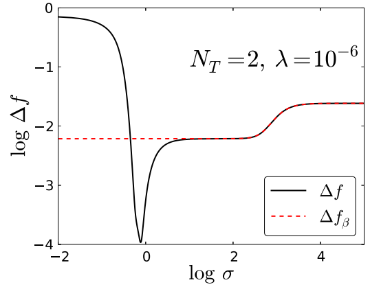
FIG. 9: Comparing the numerical \Delta f (black solid), for N_T = 2 and \lambda = 10^{-6} , with our asymptotic form \Delta f_{\beta} (red dashed) given by Eq. (30). The asymptotic form accurately recovers the behavior of \Delta f in the plateau regions, but fails for small \sigma as expected.
