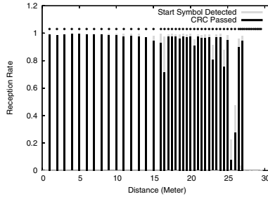
Figure 7: Spatial profile of packet delivery for \mathcal{I} , 4B6B, High Tx Power
