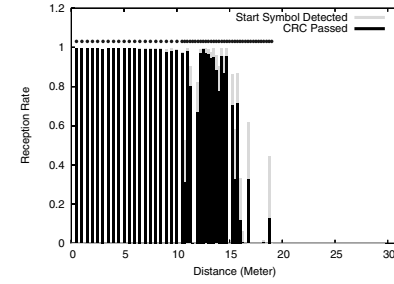
Figure 8: Spatial profile for \mathcal{O} , 4B6B, High Tx Power Figure 9: Spatial profile for \mathcal{H} , 4B6B, High Tx Power
