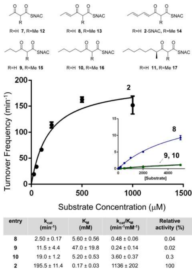
Figure 2. Full kinetic analysis of LovB MT domain towards different \beta -ketoacyl-SNAC substrates. 2 is the natural tetraketide substrate based on DML structure. 8 is the on-pathway triketide substrate of LovB. No reaction towards diketide 7 or pentaketide 11 was observed.
