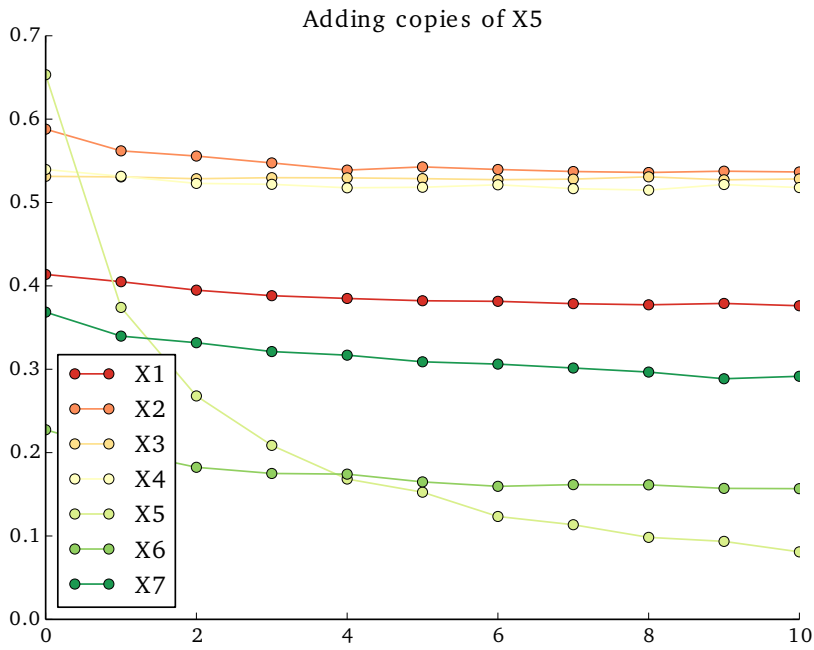
Figure 7.1: Adding copies of X_5 on the LED classification task. The more redundant variables are added, the lesser the importance of X_5 .
