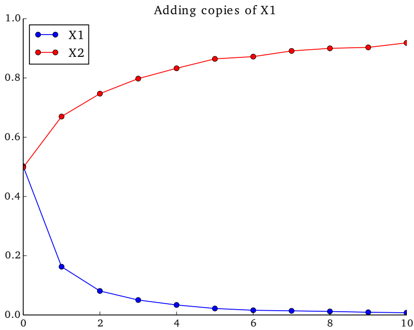
Figure 7.2: Adding copies of X_1 on a XOR classification task. The more redundant variables are added, the lesser the importance of X_1 , but the larger the importance of X_2 .
