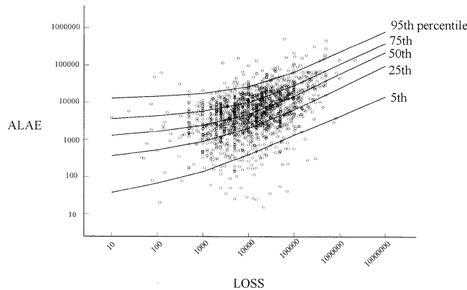
FIGURE 5 SCATTERPLOT OF ALAE VERSUS LOSS WITH QUANTILE REGRESSION CURVES SUPERIMPOSED
