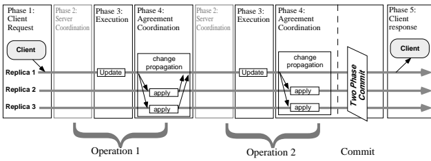
Figure 11. Eager primary copy approach for transactions
