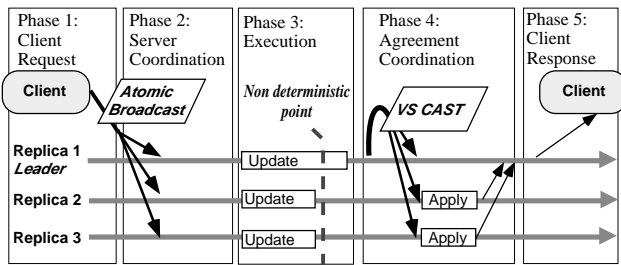
Figure 4. Semi-active replication
