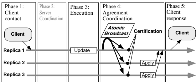
Figure 13. Certification based Database Replication
