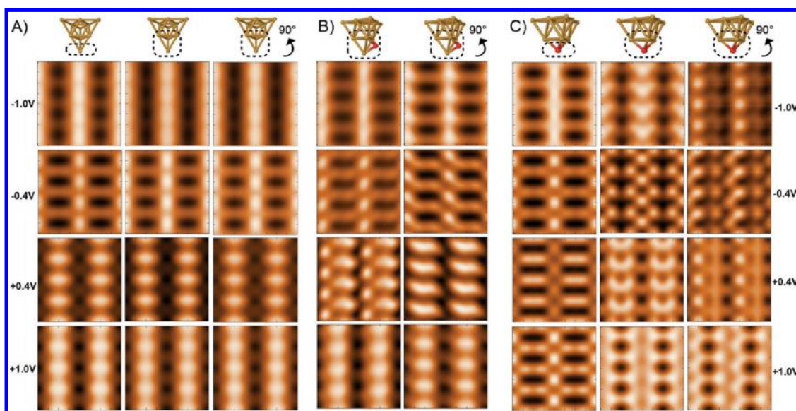
Figure 4. Current maps ( 1.44 \text{ nm} \times 1.44 \text{ nm} ) simulated for the Cu (A), the Cu–CuO (B), and the CuO (C) tips at different bias voltages and a constant tip–sample distance of d = 5 \text{ \AA} . For the calculations, tunneling currents are considered either only from the front tip atom (first columns in A and C) or by considering contributions to the tunneling current from all atoms in the double-layer apex; the tip atoms involved are encircled by dashed lines in the tip models at the top of each column. To study tip-asymmetry effects, the last column of each panel contains simulations where the tips were rotated by 90^\circ , as specified in Figure 3.
