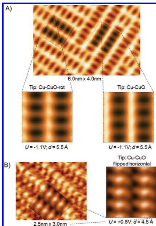
Figure 6. Comparison of experimental and simulated STM contrasts for cases where the analysis suggests Cu–CuO and Cu–CuO-rot tip configurations. The imaging parameters for the experimental constant current data were -1.10 V/ 0.40 nA (A) and +0.60 V/ 0.70 nA (B).
