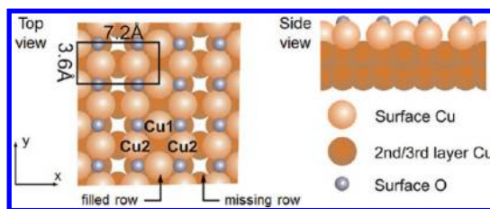
Figure 1. Schematic of the oxygen-induced missing row reconstruction of the Cu(100) surface, with the field of view reflecting the surface area covered by the simulations presented in upcoming sections. Due to the rotational symmetry of the Cu(100) surface, the x and y directions may correspond to either the [010]/[001] or the [001]/[0\bar{1}0] crystallographic directions of the substrate, respectively. The black rectangle in the top view outlines the size of the unit cell.
