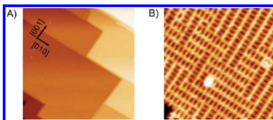
Figure 2. Experimental STM images of the Cu(100)–O surface. (A) Large-scale image ( 75\text{ nm} \times 75\text{ nm} ) revealing the step-edge pinning along the [010] and the [001] directions. (B) High-resolution image ( 9\text{ nm} \times 9\text{ nm} ) illustrating orthogonal domains also oriented along the [010] and [001] directions; note that domains may be as small as two unit cells. Imaging parameters: (A) +1.0\text{ V}/0.9\text{ nA} ; (B) -1.1\text{ V}/0.4\text{ nA} .
