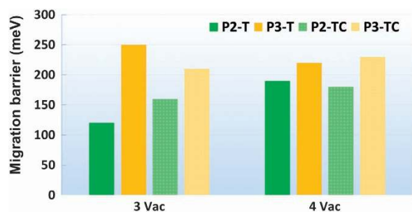
Figure 7 The calculated energy barrier of the Na-ion diffusion process for the following types: three vacancies (3 Vac) and four vacancies (4 Vac), and in NaTiO 2 (solid bars) and NaTi 0.44 Cr 0.56 O 2 (shaded bars) with layered P2 (green) and P3 (orange) structures, suggesting that the Na diffusion kinetics are determined by a structural difference (P2 vs P3) and independent of the transition metal ions.
