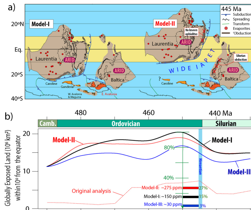
Fig. 11. (a) Late Ordovician reconstruction of the lapetus bordering continents. We place the southern margin of Laurentia at \sim 20^\circ\text{S} (Model-I, Torsvik et al., 2012) whilst Swanson-Hysell and Macdonald (2017; see their figure DR1 at 445 Ma) place Laurentia \sim 10^\circ more northward (Model-II, see supplementary section C). Thick dark brown lines in Model-II reconstruction were named 'ophiolite-bearing sutures' in Macdonald et al. (2019; see their Fig. 1 at 445 Ma) but there are no known ophiolites in Greenland and ophiolites in western Baltica were all obducted in the Silurian. This has been accounted for in Model-I reconstruction where no ophiolites in the lapetus realm were obducted within 10^\circ from the equator (yellow band). Globally, reconstruction in Swanson-Hysell and Macdonald (2017) and Macdonald et al. (2019) are identical to those of Torsvik & Cocks (2016), except for locating Laurentia 10^\circ more northward during the Ordovician (Supplementary Fig. G). This result in a much wider lapetus Ocean at 445 Ma, the Caroline Terrane has yet not collided with Laurentia and the Model-II requires fast latitudinal plate velocities ( 18\text{ cm yr}^{-1} ) to close the lapetus at around 430 Ma. (b) Exposed land globally within 10^\circ from the equator based on our Model I, Model-II (as Model-I except modified Laurentia) and Scotese (2016; Model III). All models are based on exposed land mapped out in 10 Myrs intervals in Marcilly et al. (2021) and peaks in exposed land in all models occur at 450 Ma. Swanson-Hysell and Macdonald (2017) argued for a peak in obducted arc lengths in the Late Ordovician but did not attempt to quantify the effect in terms of atmospheric CO 2 drawdown. As a simple back-of-the-envelope calculation, we estimate the effect of increased weathering by considering an obduction width of 100 km, which have been multiplied by 10 in order to account for a higher theoretical weathering efficiency (mafic versus felsic rocks) and elevated topography. Compared with the total exposed land ( 10^\circ\text{S} - 10^\circ\text{N} ) the added weathering potential can be (generously) estimated to 27% (Model-I), 15% (Model-II) and 3% (Model II). In terms of CO 2 drawdown that amounts to 275 ppm (Model-I), 150 ppm (Model-II) and 30 ppm (Model-III) in the GEOCARBSulf model. The red stippled line is based on the original estimates in Macdonald et al. (2019).
