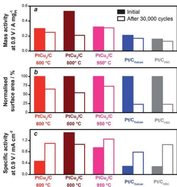
Fig. 10 Stability of dealloyed \text{PtCu}_3/\text{C} and \text{Pt}/\text{C} catalysts in a PEMFC, before and after 30 000 voltage cycles from 0.5 to 1.0 V at 100 \text{ mV s}^{-1} and 80^\circ\text{C} , adapted from data reported in Neyerlin et al. 149 (a) Mass activity, (b) surface area normalised to the initial surface area of each catalyst and (c) specific activity. For (b) and (c), the surface area was determined by the voltammetric adsorption of hydrogen between 0.5 V and 0.05 V (see footnote**). The dealloyed catalysts were based on an initial \text{PtCu}_3 precursor, which were annealed prior to dealloying at the temperatures indicated in the figure. \text{Pt}/\text{C}_{\text{Vulcan}} and \text{Pt}/\text{C}_{\text{HSC}} denote two types of commercial \text{Pt} catalysts supported on carbon, which were not annealed.
