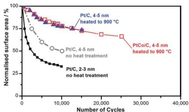
Fig. 11 Normalised surface area for different \text{Pt}/\text{C} and \text{PtCo}/\text{C} catalysts, upon cycling in a PEMFC between 0.6 and 1 V at 20 \text{ mV s}^{-1} and 80^\circ\text{C} , adapted from Makharia et al. 128 The surface area was determined by the voltammetric adsorption of hydrogen between 0.5 V and 0.05 V (see earlier footnote**).
