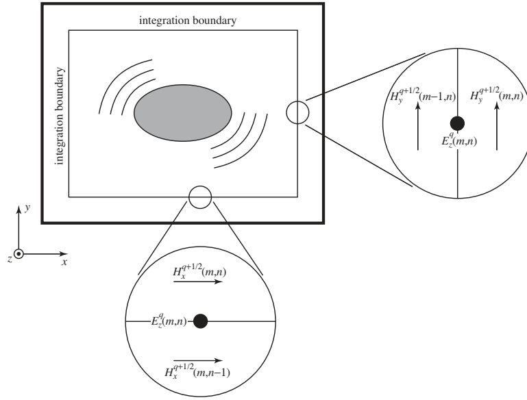
Figure 14.4: Depiction of a TM^z grid showing the integration boundary. The boundary is assumed to be aligned with electric-field nodes. The expanded views show the offset of the magnetic-field nodes from the boundary.
