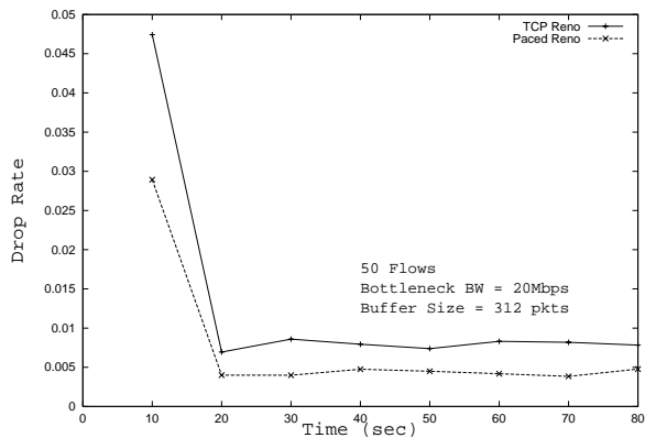
Fig. 11. Drop rate for 50 flows with variable RTTs.
