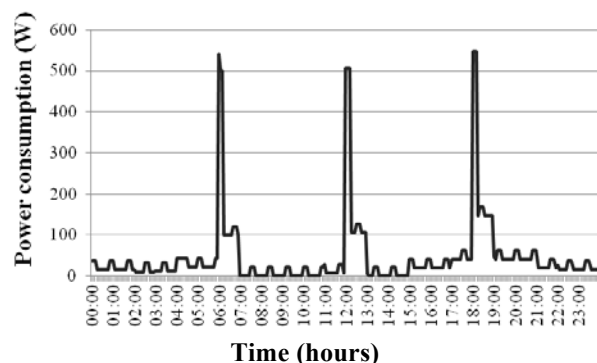
Fig. 14: High energy consumption user load profile.
