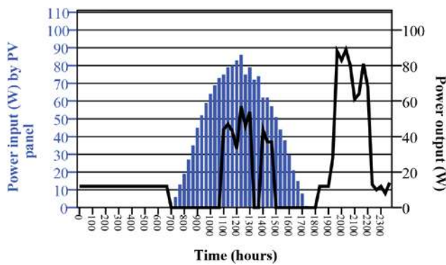
Fig. 9. Load profile and power input by solar panel on a given day of one chosen household.
