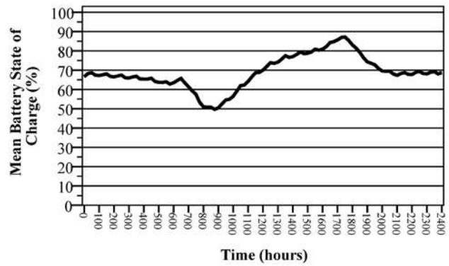
Fig. 10. Mean battery SOC of all 111 SHSs over all measured days.
