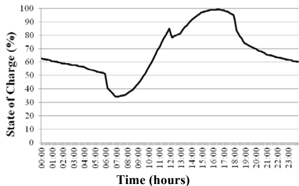
Fig. 15. Battery SOC of High energy consumption user load profile with a 200 Wp, 12V 100 Ah battery SHS, and assuming 5.5 Equivalent Sun Hours.
