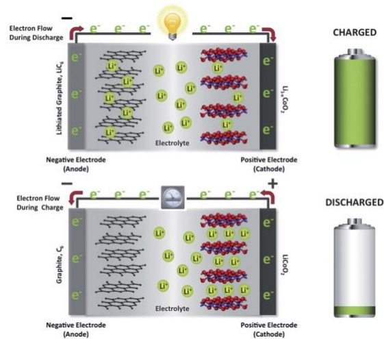
Figure 1.1 A schematic illustration of the working principle of LIBs[3]
