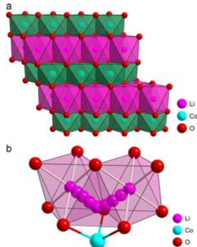
Figure 1.7 (a) Crystalline structure of layered LiCoO 2 and (b) its corresponding lithium diffusion pathways[89]
