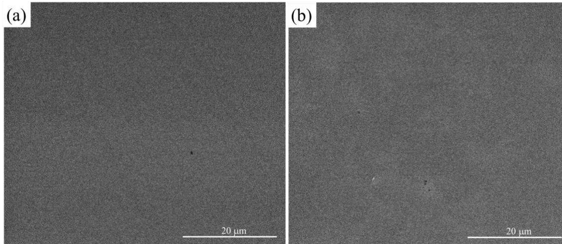
Figure 2.3 SEM images of polymeric binder film@Si wafer samples after peel test. (a) SA film@Si wafer sample; (b) PVDF film@Si wafer sample
