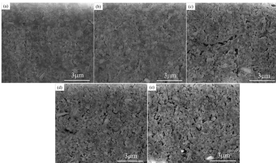
Figure 3.7 Cross sectional SEM images of Si/PAN composite electrodes: (a) fresh, (b) treated at 250°C, (c) treated at 300°C, (d) treated at 350°C, and (e) treated at 400°C
