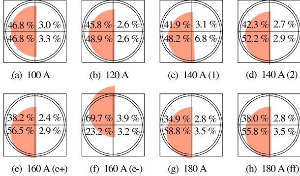
Figure 22: Representation of the distributions of positrons at the P1 quadrant detector listed in Table 5, assuming that the positrons uniformly populated a half-circular region.
