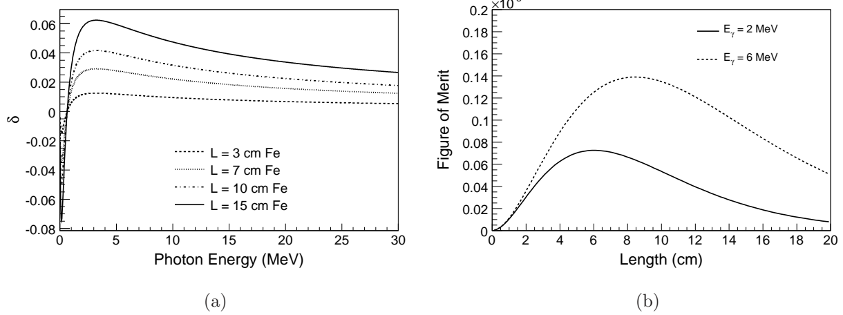
Figure 9: (a) The asymmetry \delta(E, L) defined in Eq. (9) for transmission polarimetry of fully polarized photons on MeV energy E in various lengths L of saturated iron. (b) The figure of merit \delta^2 T for 2 MeV photons (solid) and for 6 MeV photons (dashed) as a function of the length of a transmission iron polarimeter.
