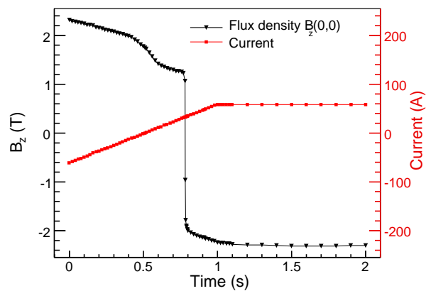
Figure 25: OPERA-2d [58] calculation of the field in magnet TP1 for a linear current ramp from -60 A to +60 A over 1 s.
