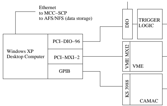
Figure 33: Layout of the DAQ hardware.
