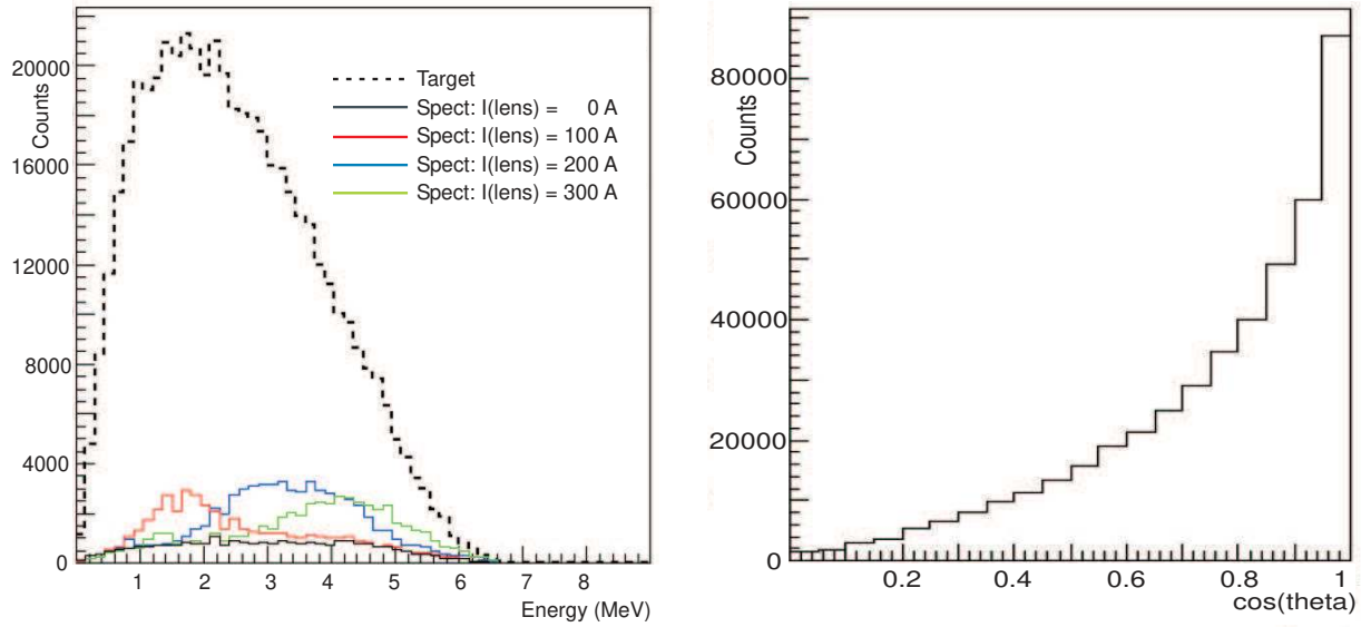
Figure 37: Simulations of focusing of positrons by the solenoid lens SL. Left: The energy spectra of positrons emerging from the production target T1 and of positrons entering the spectrometer D2 for different solenoid currents. Right: The polar angle distribution, \cos\theta , of positrons at the target exit surface.
