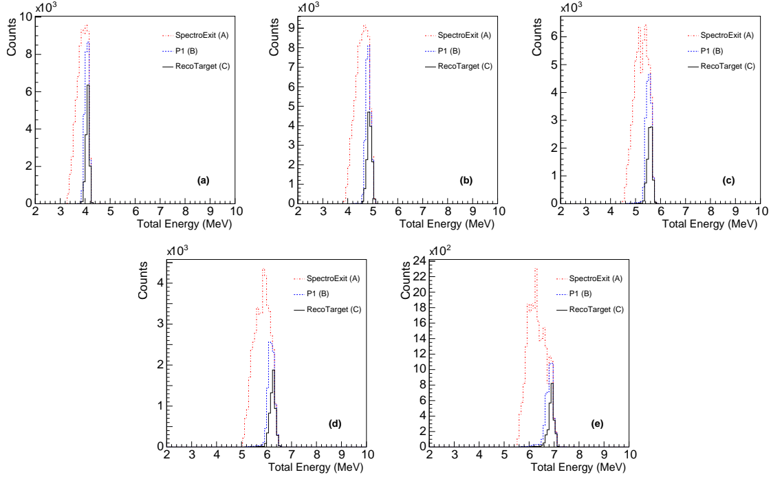
Figure 38: Simulated positron-energy spectra at the exit of the spectrometer (position A of Fig. 20), at the detector P1 (position B), and at the reconversion target T2 (position C) for the five spectrometer currents, (a): I_S = 100 A, (b): I_S = 120 A, (c): I_S = 140 A, (d): I_S = 160 A, (e): I_S = 180 A.
