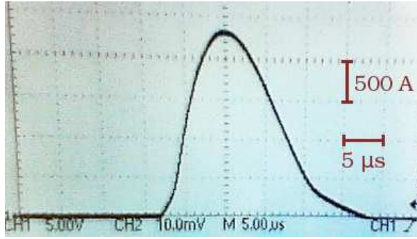
Figure 16: Current observed in the undulator shunt during a 2.3kA pulse of 12 \mu s duration.
