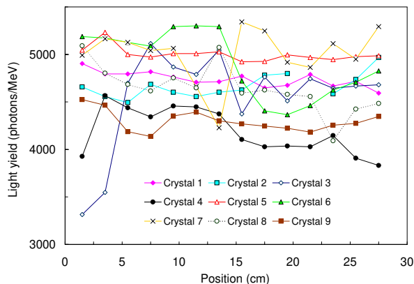
Figure 30: The photoelectron yield per MeV vs. longitudinal position for the nine CsI(Tl) crystals.
