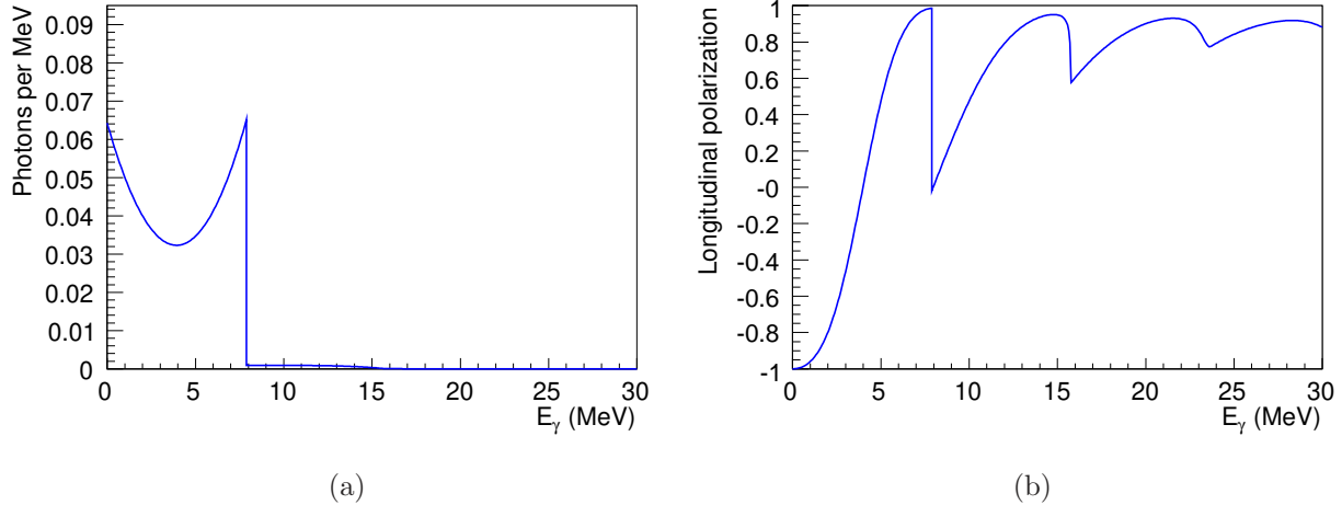
Figure 4: (a) The number spectrum N_\gamma(E) of undulator radiation as a function of photon energy E , integrated over angle, for electron energy E_e = 46.6 GeV, undulator period \lambda_u = 2.54 mm, and undulator-strength parameter K = 0.17 . The peak energy E_1 of the first-harmonic (dipole) radiation is 7.89 MeV. (b) The longitudinal polarization P_\gamma(E) of the undulator radiation as a function of photon energy for an undulator with a right-handed helical winding.
