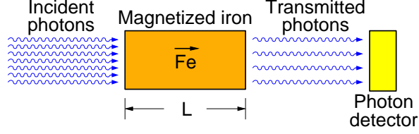
Figure 7: The concept of transmission polarimetry, in which the survival rate is measured for photons that pass through a magnetized iron absorber.
