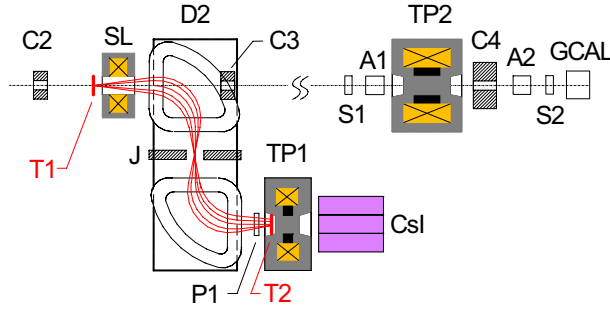
Figure 3: Schematic of the photon and positron diagnostics. A1, A2 = aerogel Cherenkov detectors, C2–C4 = collimators, D2 = dipole spectrometer magnet, Csl = 3 \times 3 array of CsI crystals, GCAL = Si-W calorimeter, J = movable W jaws, P1, S1, S2 = Si-diode detectors, SL = solenoid lens, T1 = positron-production target, T2 = reconversion target, TP1 = positron-transmission-polarimeter solenoid, TP2 = photon-transmission-polarimeter solenoid. The detectors were encased in lead and tungsten shielding (not shown).
