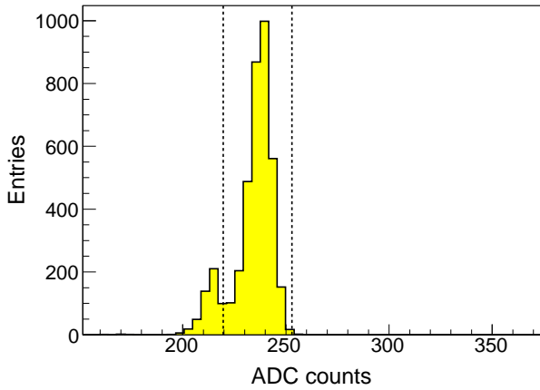
Figure 58: Example of a distribution of the beam current in toroid BT (see Fig. 2) that shows a fluctuation to low current. Only events with current within the \pm 3\sigma cuts about the mean were used in the subsequent analysis.
