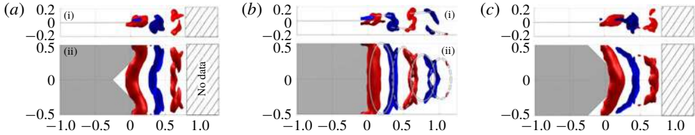
FIGURE 35. Isosurfaces of phase-averaged spanwise vorticity \langle \omega_z^* \rangle , for St = 0.2 . Red is positive, blue is negative. Spanwise (i) and panel-normal (ii) views are shown for three cases. (a–c) concave, square and convex. Adapted with permission from Van Buren et al. (2017a).
