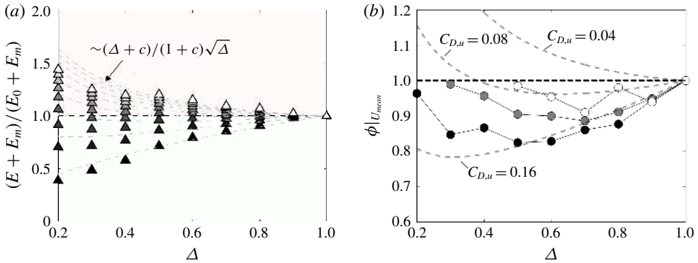
FIGURE 37. (a) Ratio of energy expended by intermittent motions to energy expended by continuous motions, including metabolic energy losses, as a function of duty cycle for \theta_0 = 15^\circ , all frequencies, with C_{Db} = 0.1 . Each point is an average over all frequencies. The shading denotes the value of the metabolic power fraction c_m , 0 to 2 in intervals of 0.25 (dark to light). (b) Ratio of energy expended by intermittent motions to energy expended by continuous motions, restricted to equal mean speeds. Dashed lines correspond to the model. The symbol grey scale corresponds to three values of (dimensional) mean speed chosen, U_{mean} = 0.2, 0.25, 0.3 (dark to light). The frequency of the intermittent motion was chosen so that it would have a speed equal to the continuous motion. Reproduction with permission from Floryan et al. (2017b).
