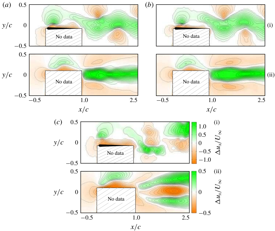
FIGURE 41. Heaving foil. (i) Phase- and (ii) time-averaged change in streamwise velocity ( h/c = 12.5\% , St = 0.4 ). Waveform: (a) triangular-like \kappa = -0.99 ; (b) sinusoidal \kappa = 0 ; (c) square-like \kappa = 0.99 . Reproduction with permission from Van Buren et al. (2017b).
