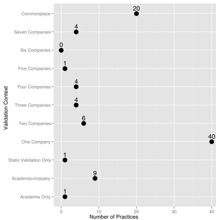
Fig. 3 Validation Context
