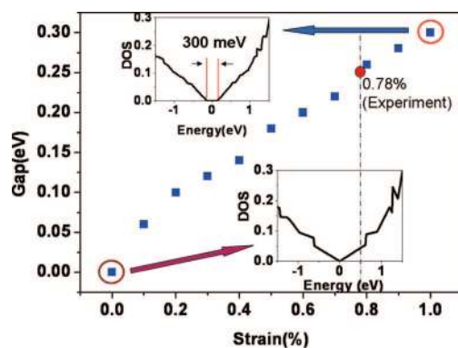
Figure 5. Band gap of strained graphene with the increase of uniaxial tensile strain on graphene. The magnitude of the gap is determined by the gap opening of the density of states. The insets show the calculated density of states (DOS) of unstrained and 1% tensile strained graphene. The dashed line and red solid dot indicate the calculated band gap of graphene under the highest strain (0.78%) in our experiment.
