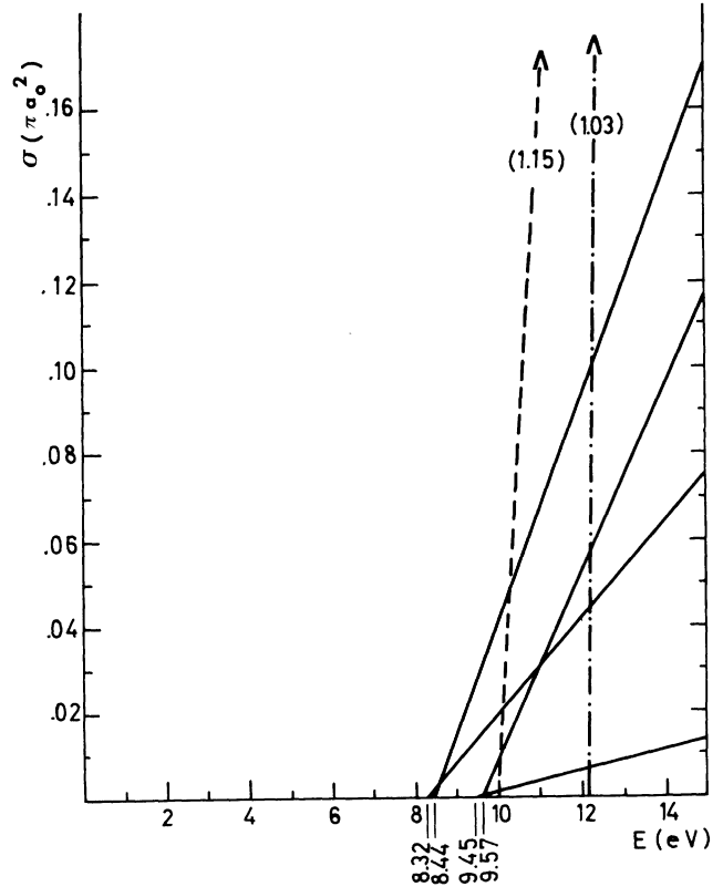
Fig. 3 - — Electron impact excitation cross sections for the first four excited states of Xe. --- Electron impact excitation cross-section for Xe (pseudo state at 10 eV). -.- Electron impact ionization cross-section for Xe.
