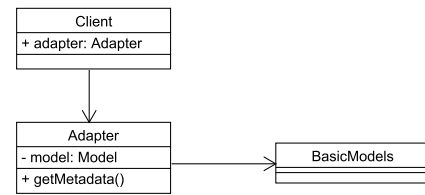
Fig. 5. Adapter Pattern
