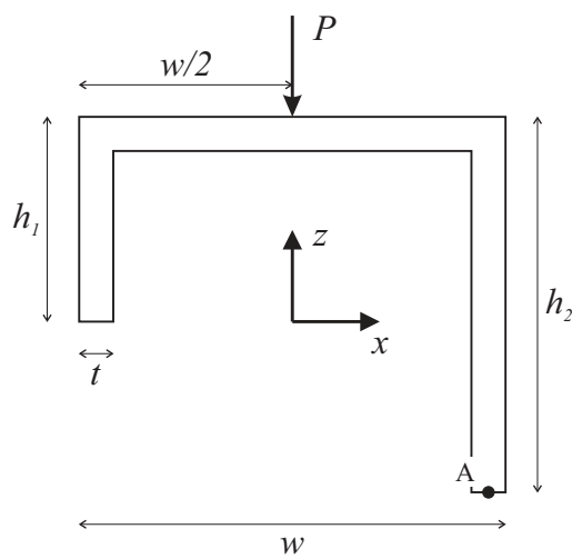
Figure 10: Cross-section geometry of the unsymmetric channel beam and loading condition.
