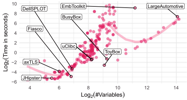
Fig. 17 Time it took to compute the distribution of SAT-solutions for all models in the benchmark
