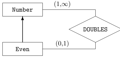
Figure 5: The ER schema corresponding to Example 2.2
