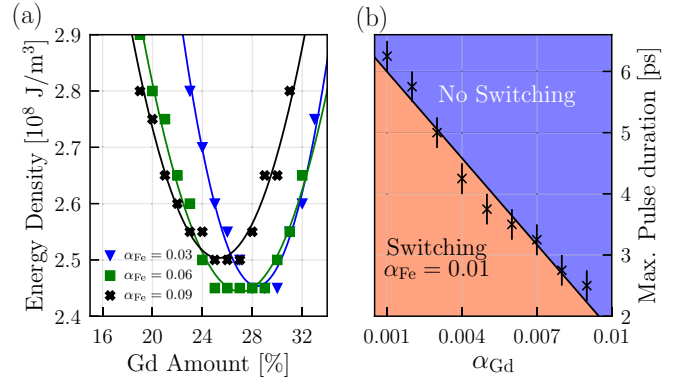
FIG. 4. Simulation results for (a) critical laser fluence of a 350-fs pulse as function of the Gd concentration ( \alpha_{\text{Gd}} = 0.01 constant) for \alpha_{\text{Fe}} = 0.03 (blue triangles), 0.06 (green boxes), 0.09 (black crosses). The lines represent an x^2 fitting and serve only as a guide to the eye. (b) Maximum pulse duration achieved in the model as function of the Gd damping \alpha_{\text{Gd}} ( \alpha_{\text{Fe}} = 0.01 constant) for an \text{Fe}_{75}\text{Gd}_{25} alloy.
