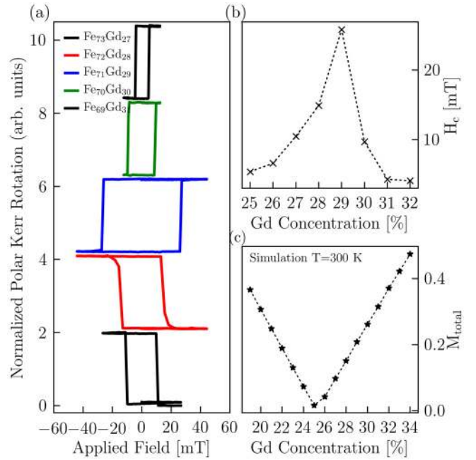
FIG. 1. (a) Magnetic hysteresis of different Fe-Gd alloys between 27%–31% gadolinium probed by the magneto-optical Kerr rotation at 300 K. The use of an objective lens that is close to the electromagnet’s gap induces an additional slope on the Kerr hysteresis data, due to a Faraday effect in the lenses’ glass. This slope, which is independent of the sample, was numerically removed from this figure. The polarity of the hysteresis changes as the system crosses the compensation. The coercivity diverges as the Gd concentration approaches the compensation point. (b) The experimentally measured coercive field H_c of (a) as function of the Gd concentration. The line is guidance to the eye. (c) The simulated total magnetization of the Fe-Gd alloy at 300 K as function of the Gd concentration. The simulated magnetization compensation temperature is slightly lower (between 25%–26%) than the experimental one with the drawn line being guidance to the eye.
