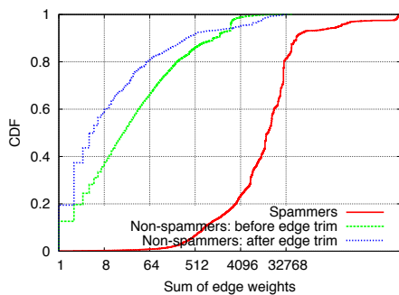
(b) CDF of edge-weight-sum in user-link graph
