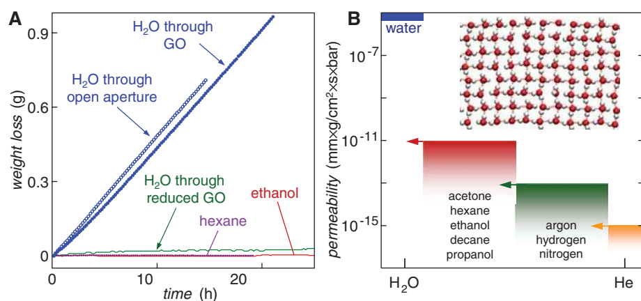
Fig. 2. Permeation through GO. (A) Weight loss for a container sealed with a GO film ( h \approx 1 \mu m; aperture's area \approx 1 cm 2 ). No loss was detected for ethanol, hexane, etc. (7), but water evaporated from the container as freely as through an open aperture (blue curves). The measurements were carried out at room temperature in zero humidity. (B) Permeability of GO paper with respect to water and various small molecules (arrows indicate the upper limits set by our experiments). (Inset) Schematic representation of the structure of monolayer water inside a graphene capillary with d = 7 Å, as found in our MD simulations (7).
